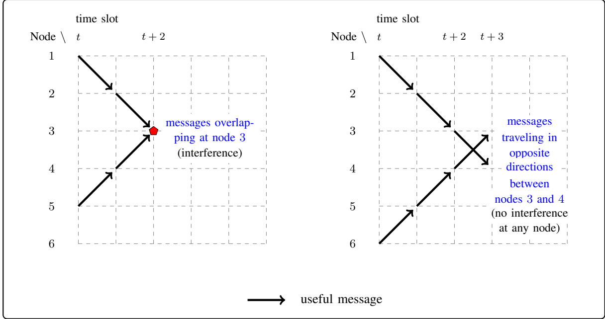
Fig. 3. Depiction of the state of 6-node network in the case where node-pairs (1,5) and (1,6) are broadcasting at the same time slot
