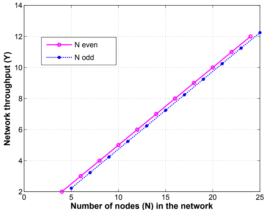
Fig. 4. Network throughput for schedules generated using Algorithm 2 for various N \leq 25 . The throughput consistently achieves the bounds for both even and odd N .
