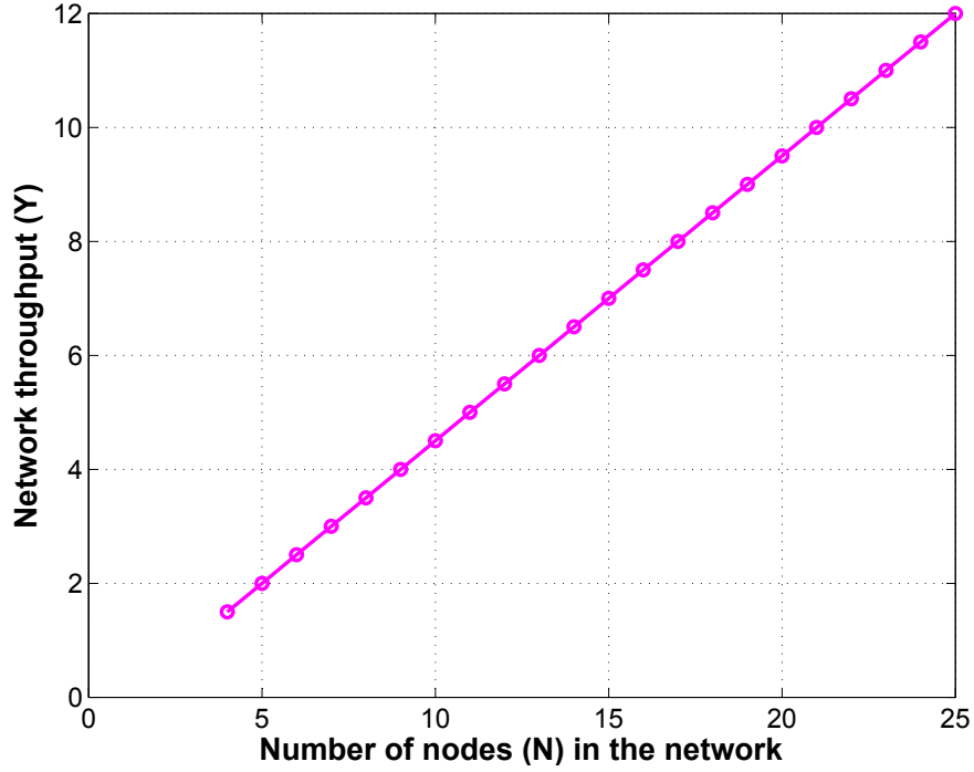
Fig. 6. Network throughput for schedules generated using Algorithm 3 for various N \leq 25 . The throughput consistently achieves the bound (N-1)/2 .
