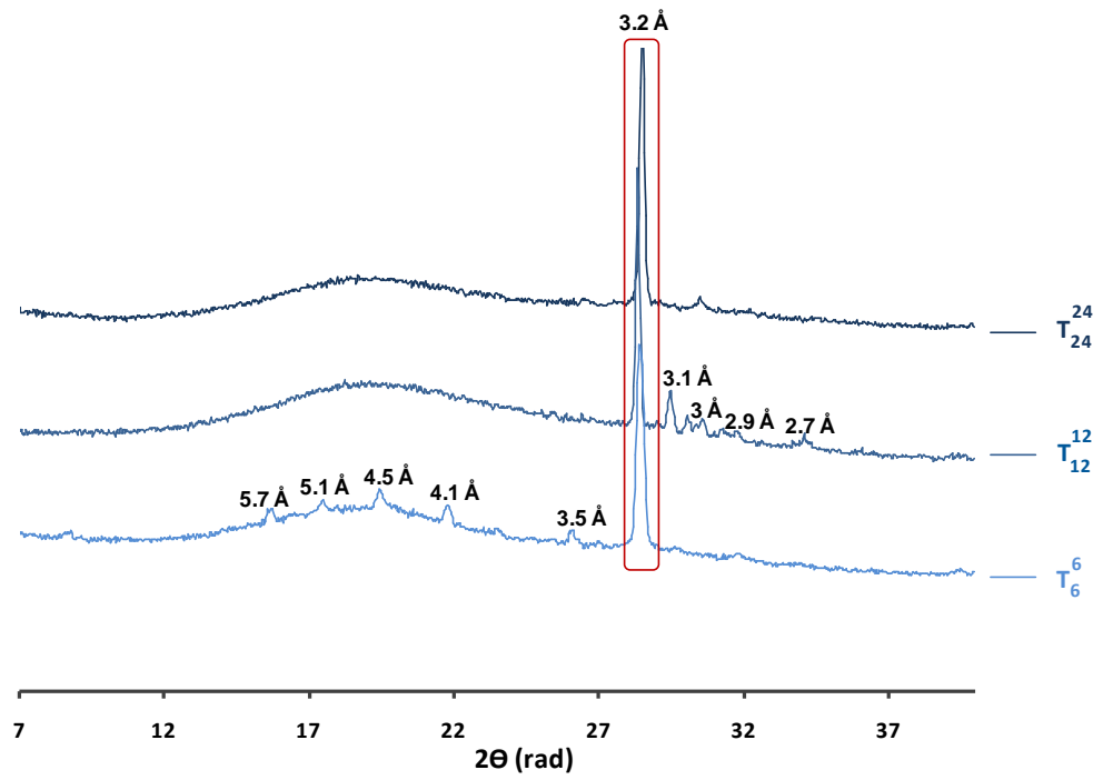
Figure 6: X-ray diffraction patterns measured by powder method for T 6 , T 12 and T 24 .
