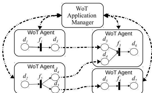
Figure 4: WoT Application Deployment
