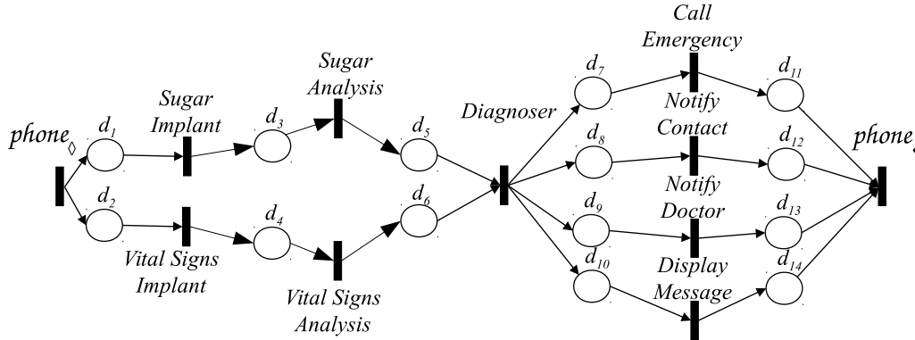
Figure 5: Case Study: the e-Health WoT application
