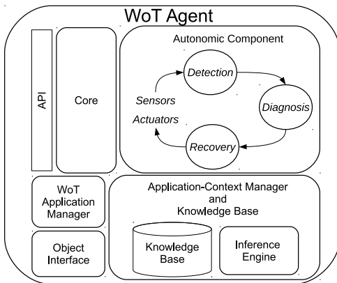
Figure 1: WoT Agent Architecture
