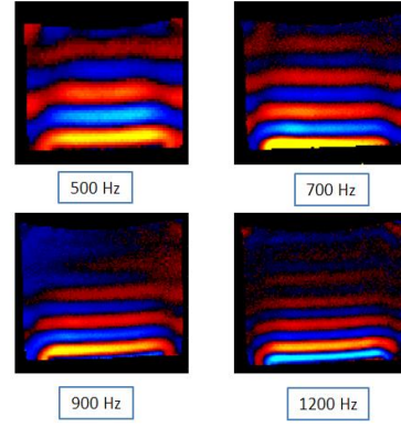
Figure 2. Wave images for phantom (A) at different excitation frequencies: 500, 700, 900 and 1200 Hz.
