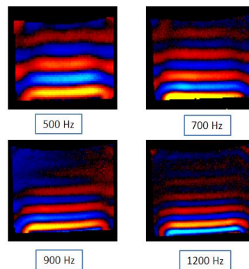
Figure 2. Wave images for phantom (A) at different excitation frequencies: 500, 700, 900 and 1200 Hz.
