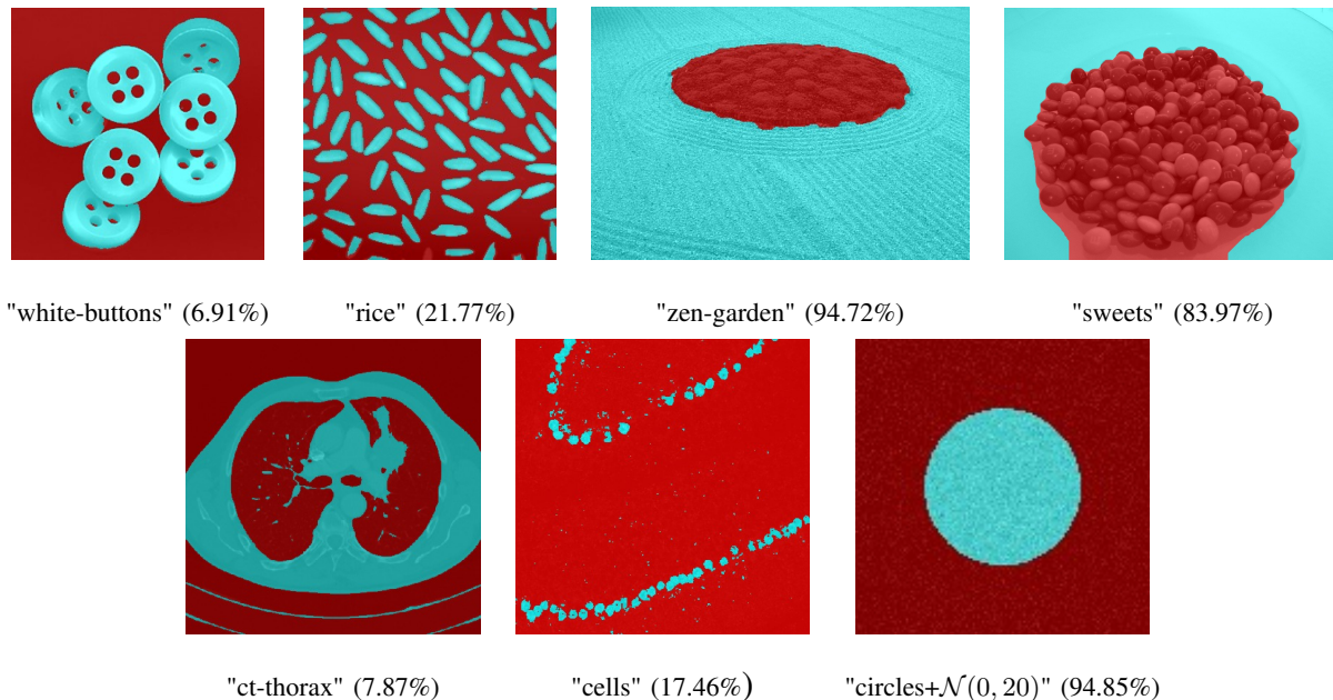
Fig. 7: Segmentation results using a TV+L^2 model in connectivity 1. The segmentation is superimposed on the original image by transparency. The minimal relative size of the reduced graph is indicated in parenthesis below each image.
