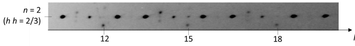
FIG. 1. Superlattice diffraction spots along (2/3 \ 2/3 \ l) line.
