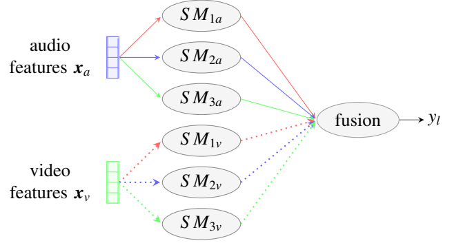
Figure 3: Strength Modelling (SM) with late fusion strategy. Fused predictions are from multiple independent modalities with the same model (denoted by the red, green, or blue lines), multiple independent models within the same modality (denoted by the solid or dotted lines), or the combination.
