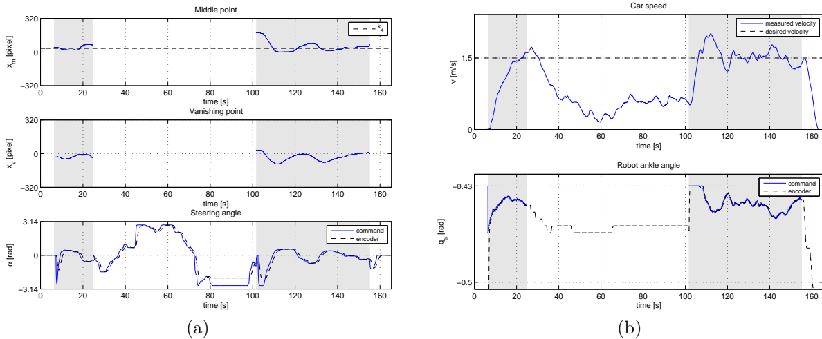
Figure 14: Second experiment: switching between teleoperated and autonomous modes. (a) Middle point abscissa x_m (top), vanishing point abscissa x_v (center), and steering angle \alpha (bottom). (b) Car speed v (top) and ankle joint angle q_a (bottom).
