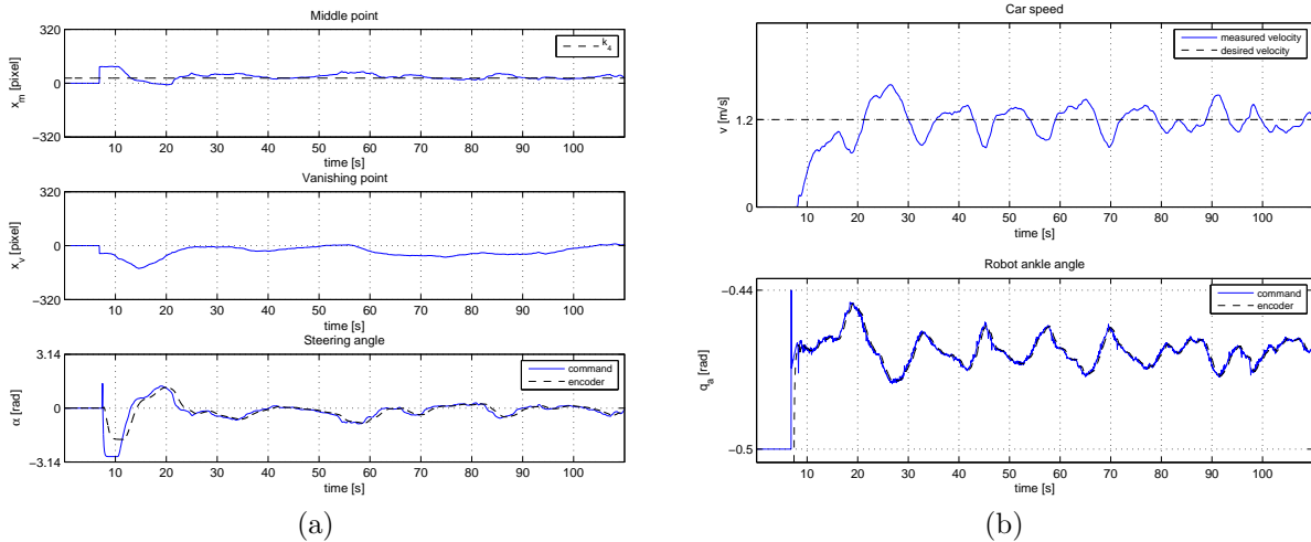
Figure 12: First experiment: autonomous car driving. (a) Middle point abscissa x_m (top), vanishing point abscissa x_v (center), and steering angle \alpha (bottom). (b) Car speed v (top), already shown in fig 10, and ankle joint angle q_a (bottom).
