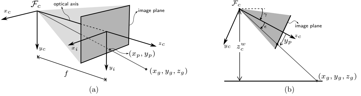
Figure 7: Schematic representation of the robot camera looking at the road. (a) Any visible cartesian point (x_g, y_g, z_g) on the ground has a projection on the camera image plane, whose coordinates expressed in pixels are (x_p, y_p) . (b) The measurement of this point on the image plane, together with the camera configuration parameters, can be used to estimate the depth z_g of the point.
