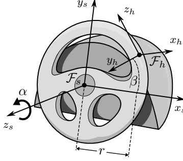
Figure 3: The steering wheel, with rotation angle \alpha , hand and steering frames, \mathcal{F}_h and \mathcal{F}_s . The parameters r , the radius of the wheel, and \beta , characterizing the grasp configuration, are also shown here.
