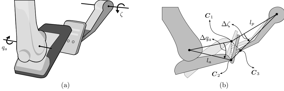
Figure 4: (a) The robot foot operates the gas pedal by regulating the joint angle at the ankle q_a , to set a pedal angle \zeta , and yield car acceleration a . (b) Geometric relationship between the ankle and the gas pedal angles.
