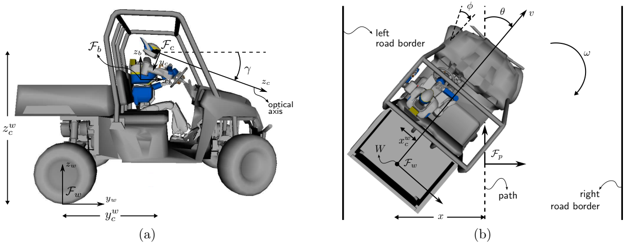
Figure 2: Side (a) and top view (b) of a humanoid robot driving a car with relevant variables.
