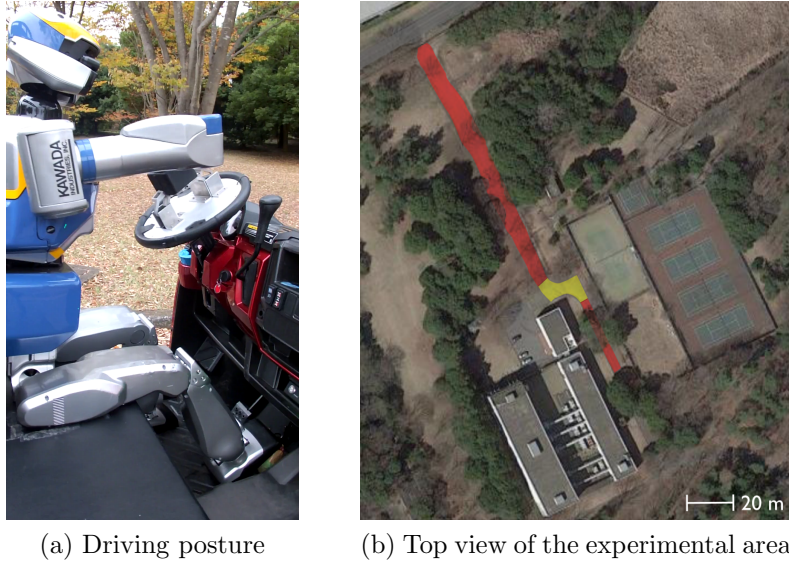
Figure 9: The posture taken by HRP-2Kai during the experiments (a) and the experimental area at the AIST campus (b).
