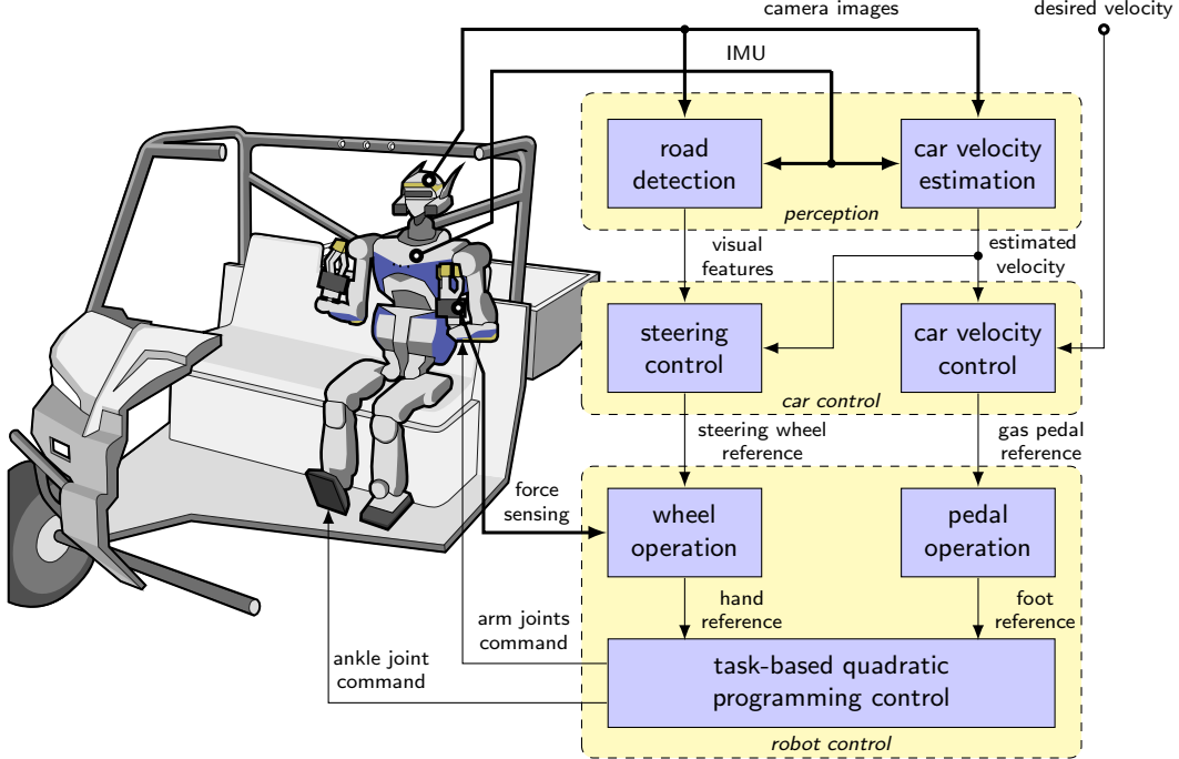
Figure 1: Conceptual block diagram of the driving framework.
