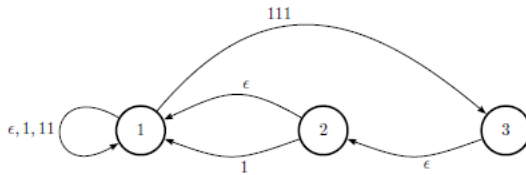
FIGURE 15. Prefix automaton of \sigma .
