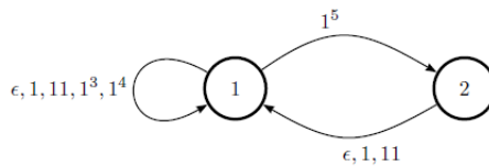
FIGURE 8. Prefix automaton of \sigma .
