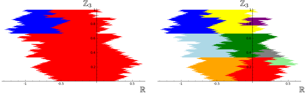
FIGURE 9. The central tile \mathcal{R}_{\sigma} divided in the red (light gray) subtile \mathcal{R}_{\sigma}(1) and the blue (dark gray) subtile \mathcal{R}_{\sigma}(2) , and the self similar structure arising from the set equations.
