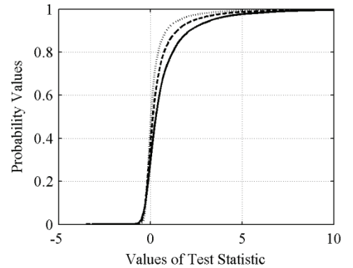
Figure 1. Empirical cdf associated with different data window lengths. L_w = 4 (dotted line). L_w = 7 (dashed line). L_w = 11 (solid line).
