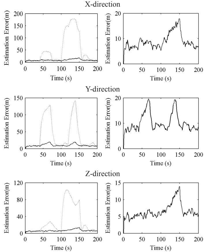
Figure 5. RMSEs of positioning estimations in three directions (50 MC runs). The proposed approach (solid line). The standard EKF (dotted line).
