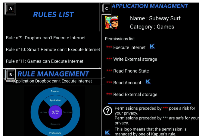
Fig. 2. Rule management interface
