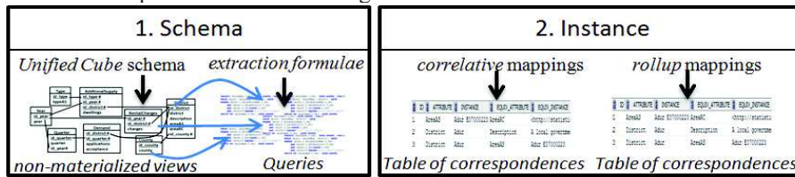
Fig. 4. Implementation framework for Unified Cubes
