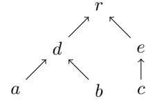
Fig. 3. O = (\preceq, C) example of ordering of concepts
