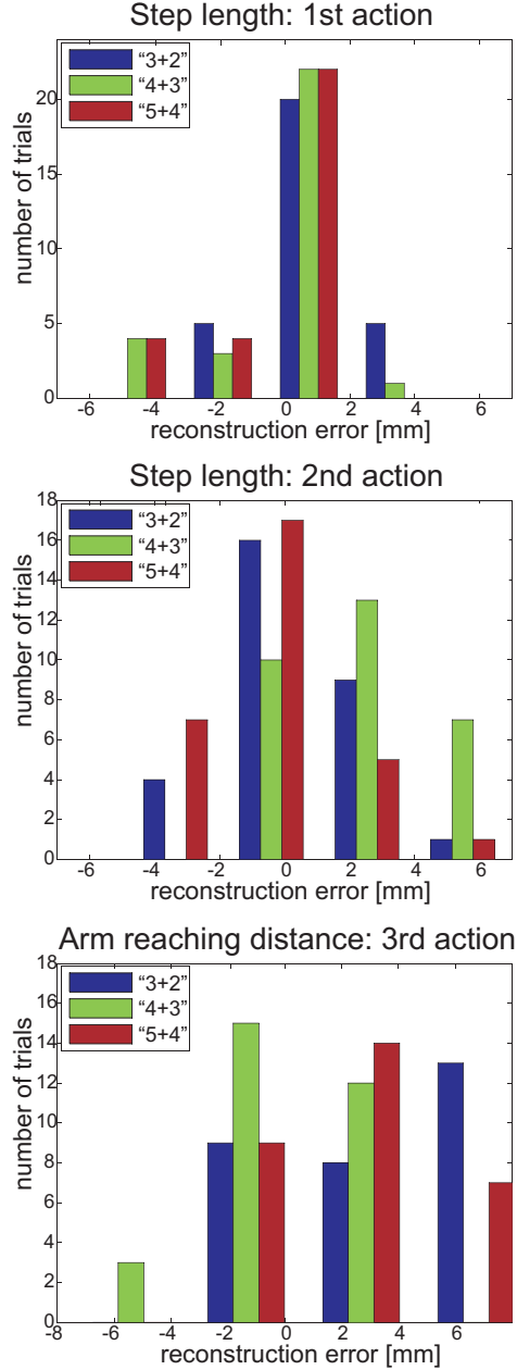
Figure 9: Reconstruction accuracy of the step-sizes and reaching goal distances for different numbers of sources. The figure shows the histograms of the spatial errors. The first number indicates the number of sources learned from the first step (action 1), and the second number the number of sources used to approximate the residuals of the other actions (2 and 3).
