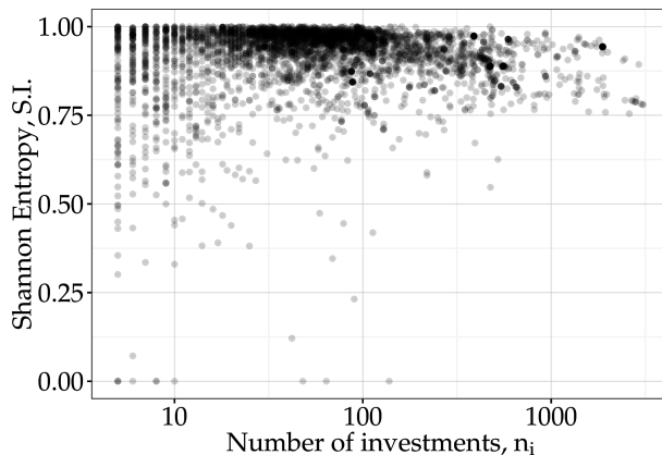
Figure 2: Shannon Entropy S_i as a function of the number of investments n_i , each dot represents a single fund.
