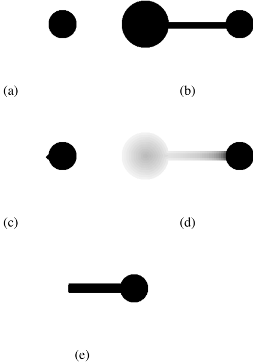
Fig. 5. (a) Set X . (b) Set Y (c) The median calculated according to (39). (d) The grey scale image obtained by Meyer's method. (e) Median calculated using the proposed approach (47).
