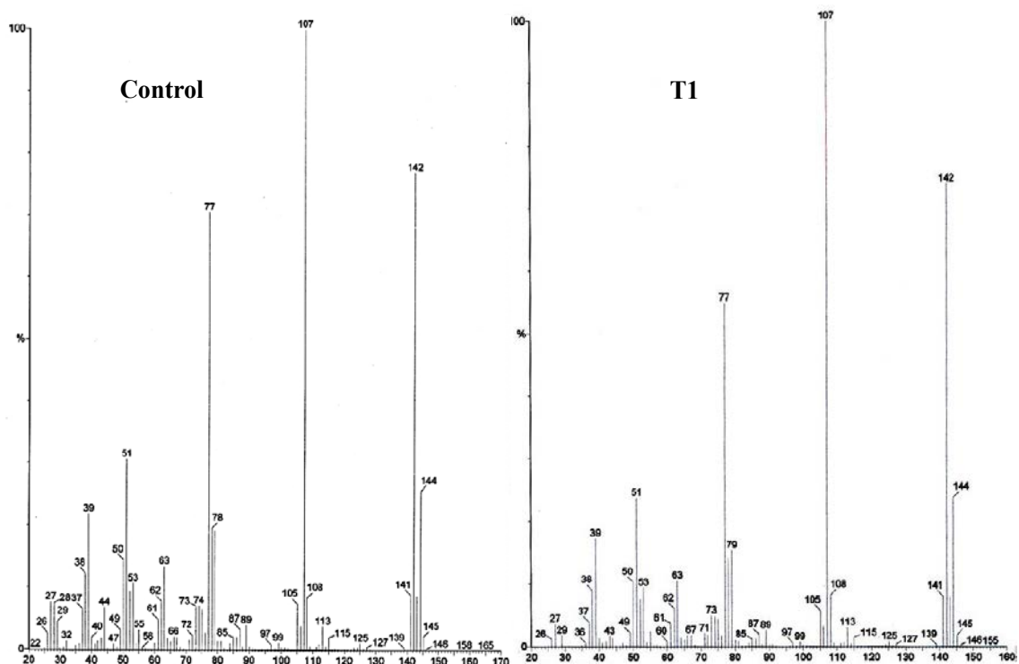
Figure 6a: GC-MS spectra of control and treated (T1) samples of p -chloro- m -cresol.
