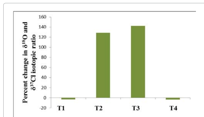
Figure 8: Percent change in \delta^{18}\text{O} and \delta^{37}\text{Cl} isotopic ratio in treated samples as compared to control.
