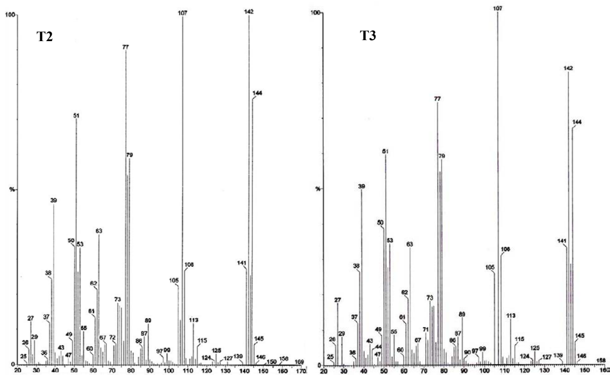
Figure 6b: GC-MS spectra of treated (T2 and T3) samples of p -chloro- m -cresol.
