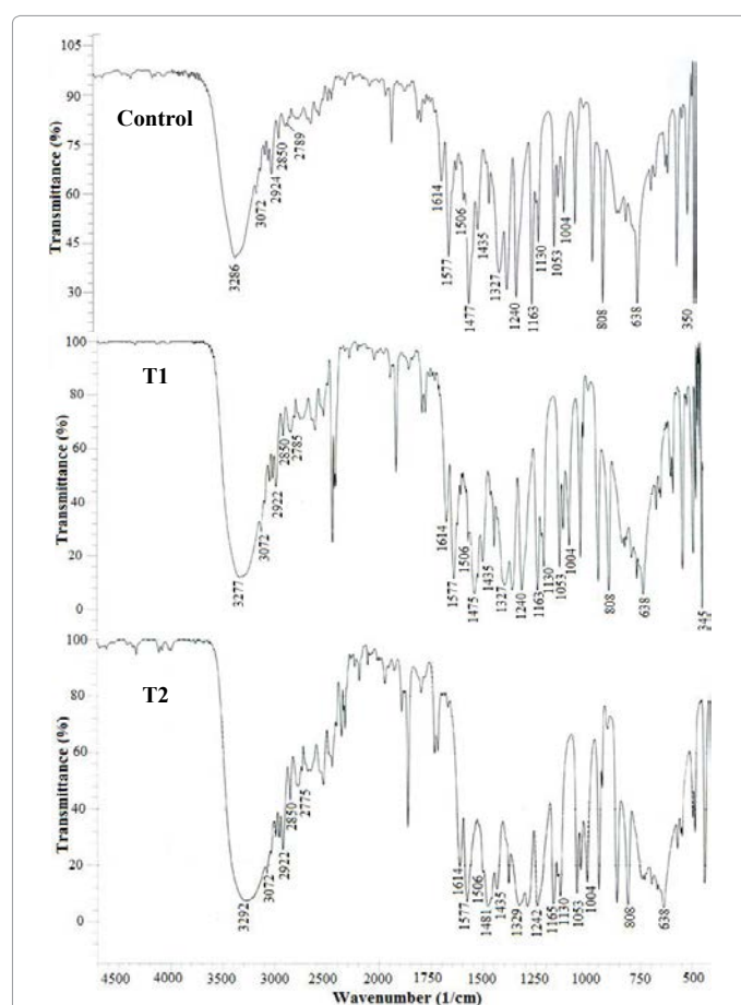
Figure 4: FT-IR spectra of control and treated (T1 and T2) samples of p -chloro- m -cresol.
