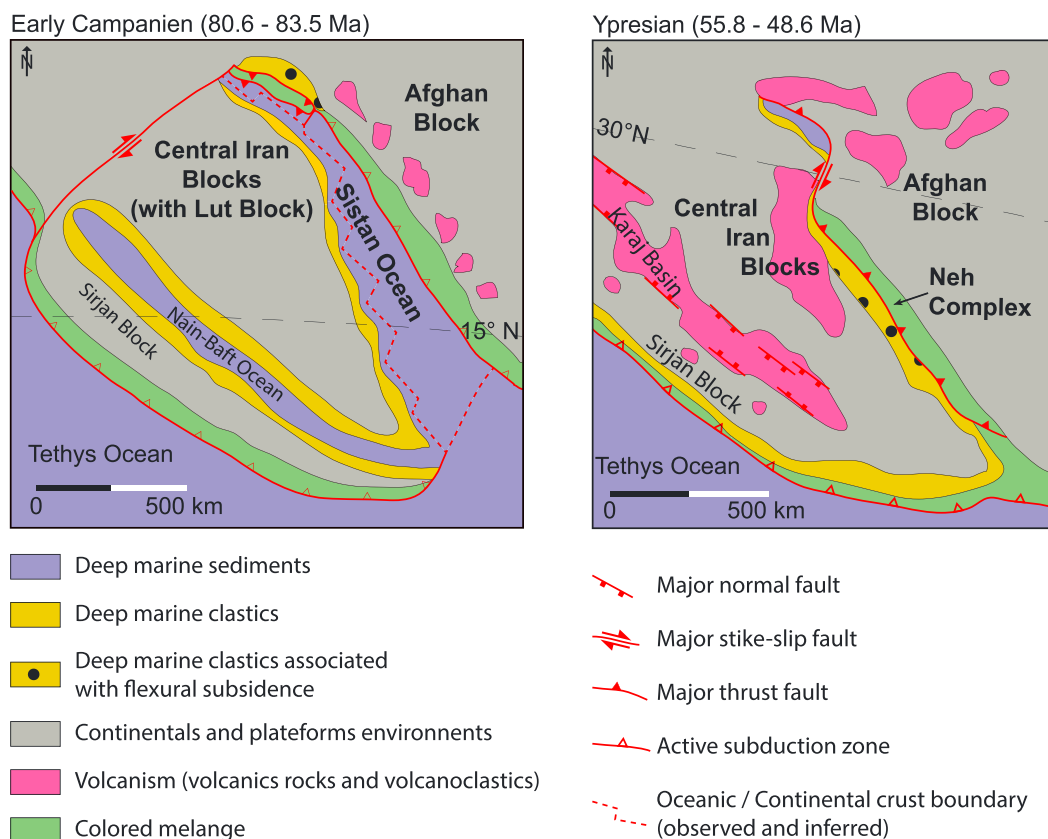
Figure 3. Tectonic Plates reconstruction for the Central Iran in early Campanian and Ypresian [modified from Barrier and Vrielynck, 2008].
