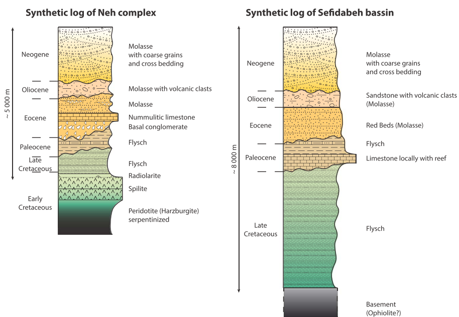
Figure 4. Synthetic logs of Neh complex and Sefidabeh basin.
