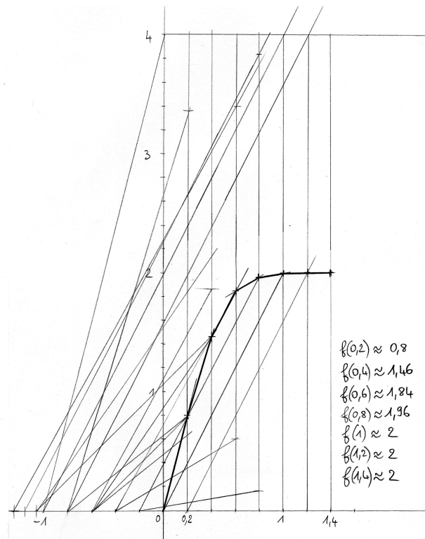
Figure 7.8. A construction of the equation y' = 4 - y^2 with y(0) = 0 .
