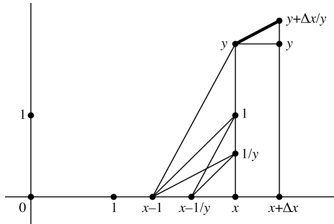
Figure 7.5. Basic construction of a tangent for the equation y' = 1/y .
