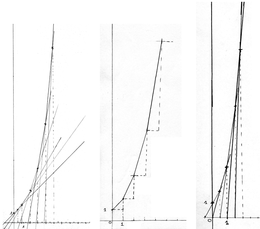
Figure 7.3. Three constructions of the exponential.
