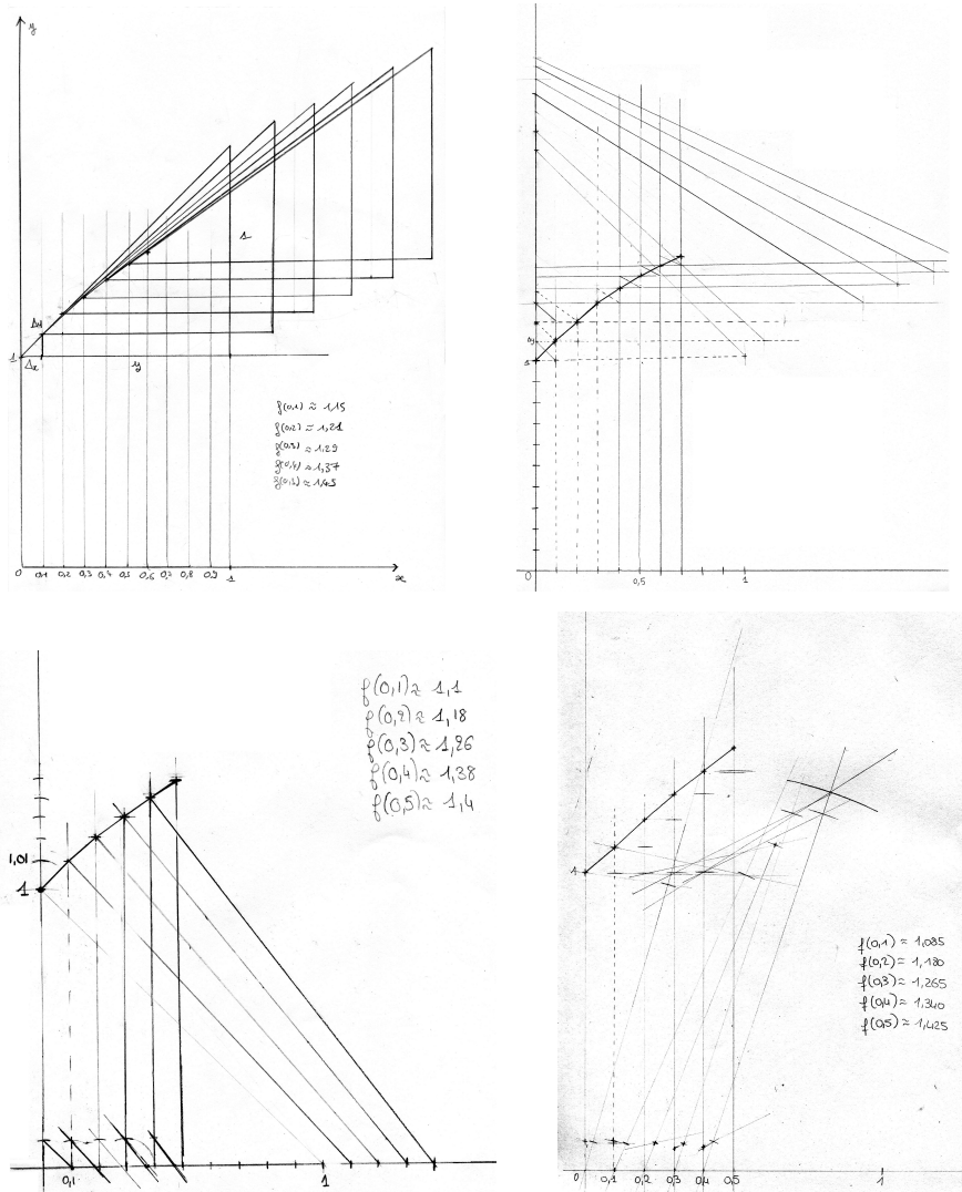
Figure 7.6. Four constructions of the equation y' = 1/y with y(0) = 1 .
