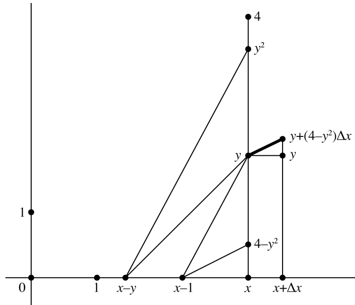
Figure 7.7. Basic construction of a tangent for the equation y' = 4 - y^2 .
