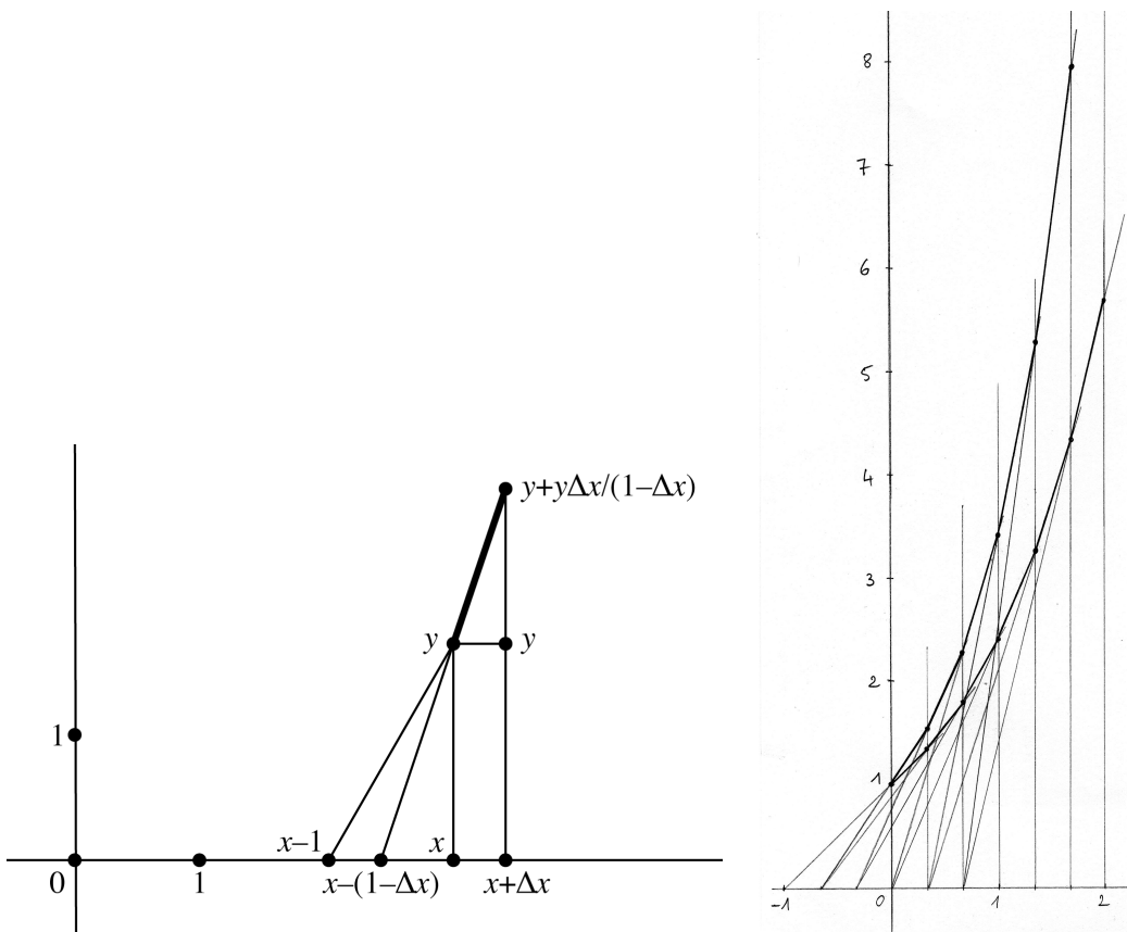
Figure 7.4. Constructing the exponential using Euler's implicit method.
