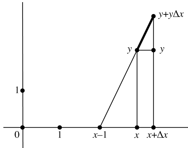
Figure 7.2. Basic construction of a tangent to the exponential.
