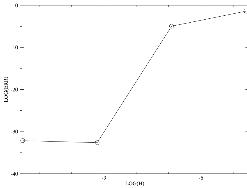
Figure 14: Convergence in L_1 norm - \tau_0 = 10^{-6} - Shock wave including void fraction disequilibrium circles S_{UPW1}
