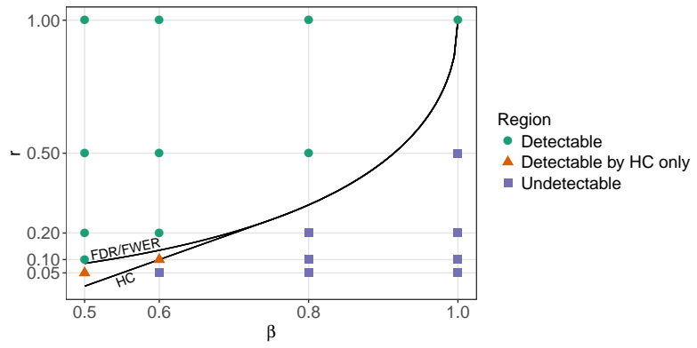
FIG 9. Top: detection power of JER controlling procedures for independent test statistics in the sparsity range for 4 \times 5 parameter configurations for (\beta, r) in the sparsity range [1/2, 1] \times [0, 1] . Bottom: these 4 \times 5 configurations are positioned with respect to the detection boundaries identified in Donoho and Jin (2004).
