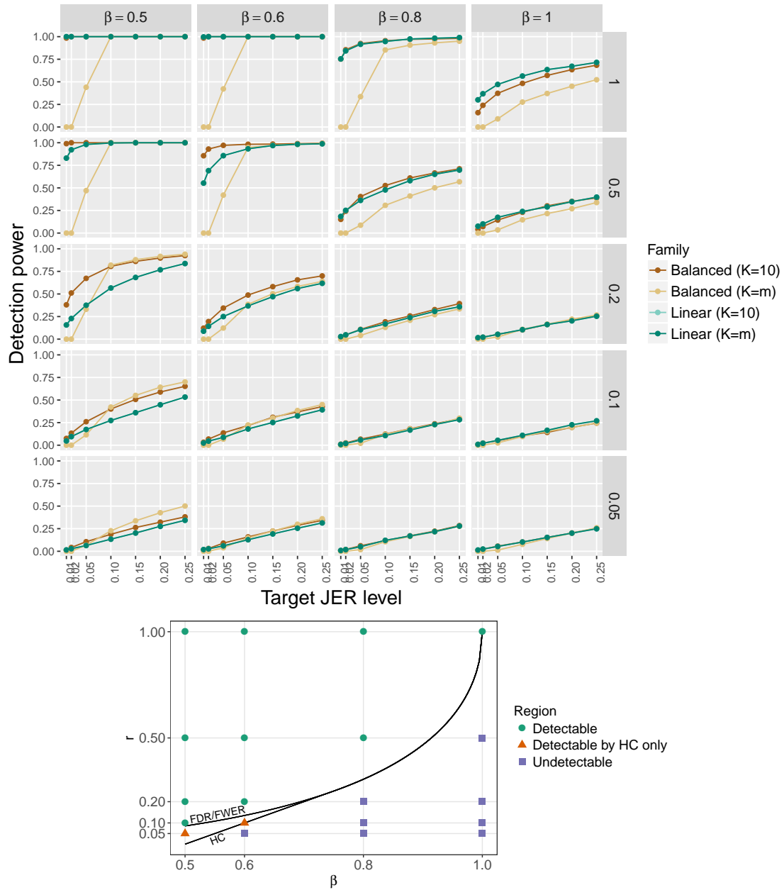
FIG 9. Top: detection power of JER controlling procedures for independent test statistics in the sparsity range for 4 \times 5 parameter configurations for (\beta, r) in the sparsity range [1/2, 1] \times [0, 1] . Bottom: these 4 \times 5 configurations are positioned with respect to the detection boundaries identified in Donoho and Jin (2004).
