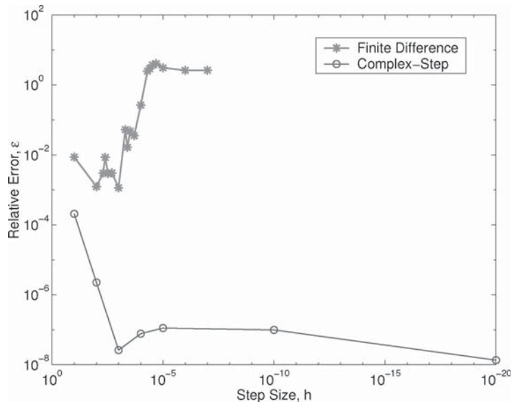
Fig. 6. Convergence of gradients as step size is decreased. \epsilon = (|f - f_{ref}|)/|f_{ref}| ; reference is complex-step result at h = 10^{-30} .
