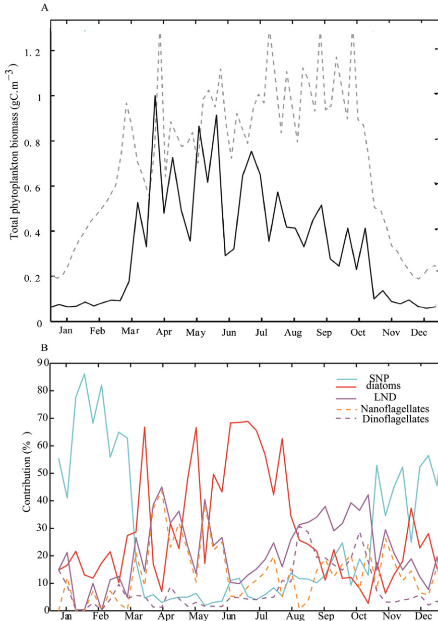
Fig. 14. (A) Seasonal evolution (5 days average) of total phytoplankton biomass at SOMLIT Brest station (Ste Anne du Portzic (48°21' N; -4°33' W) (solid black line) and in the surface layer of the modeled well-mixed area (cluster A; dashed black line). (B) Composition of the phytoplankton assemblages in SOMLIT data (% of total biomass) (solid blue line: picoeukaryotes + Synechococcus sp., solid red line: diatoms, solid purple line: nanoflagellates + dinoflagellates, dotted orange line: nanoflagellates only and dotted purple line: dinoflagellates only). These curves are obtained by compiling different years of data (1998 to 2012).
