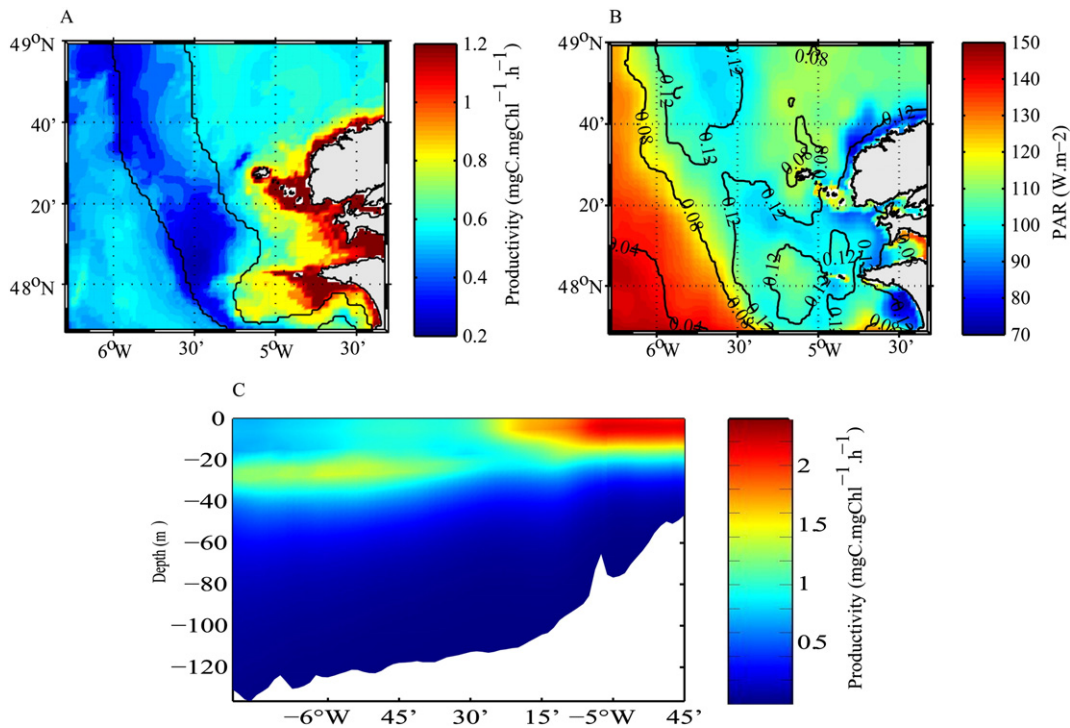
Fig. 8. (A) Vertically averaged assimilation number during the summer with limits of the three clusters coming from the k-means analysis (August–September average). (B) 0–20 m average Photosynthetic Available Radiation (contours are total phytoplankton biomass ( \text{gC}\cdot\text{m}^{-2} )). (C) Vertical distribution of assimilation number along the 48°08' N transect (see Fig. 1) in September.
