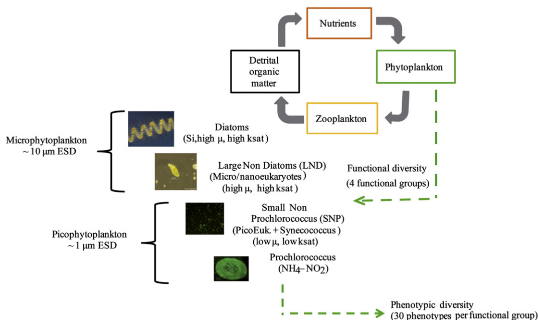
Fig. 2. Conceptual scheme of the biogeochemical model and its representation of phytoplanktonic diversity. (ESD) equivalent spherical diameter, ( \mu ) maximum growth rate, (ksat) nutrient half-saturation constants.
