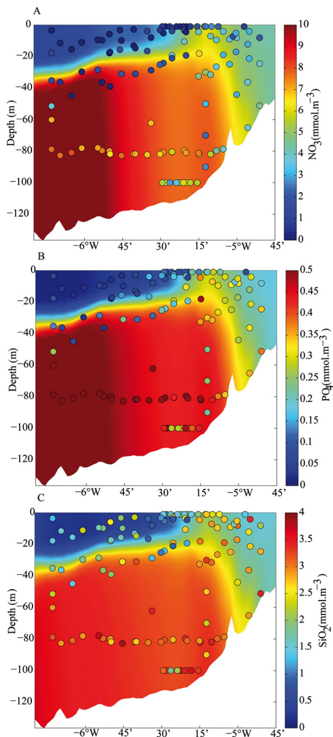
Fig. 6. In-situ concentrations of main macronutrients (A) nitrates; (B) phosphate and (C) silicates (scattered circles) sampled during the FroMVar cruises (September 13 to September 15, 2007 and 19 to 29 September 2009) superimposed to simulated summer concentrations (August–September average) along the 48^{\circ}08' N transect (see Fig. 1).
