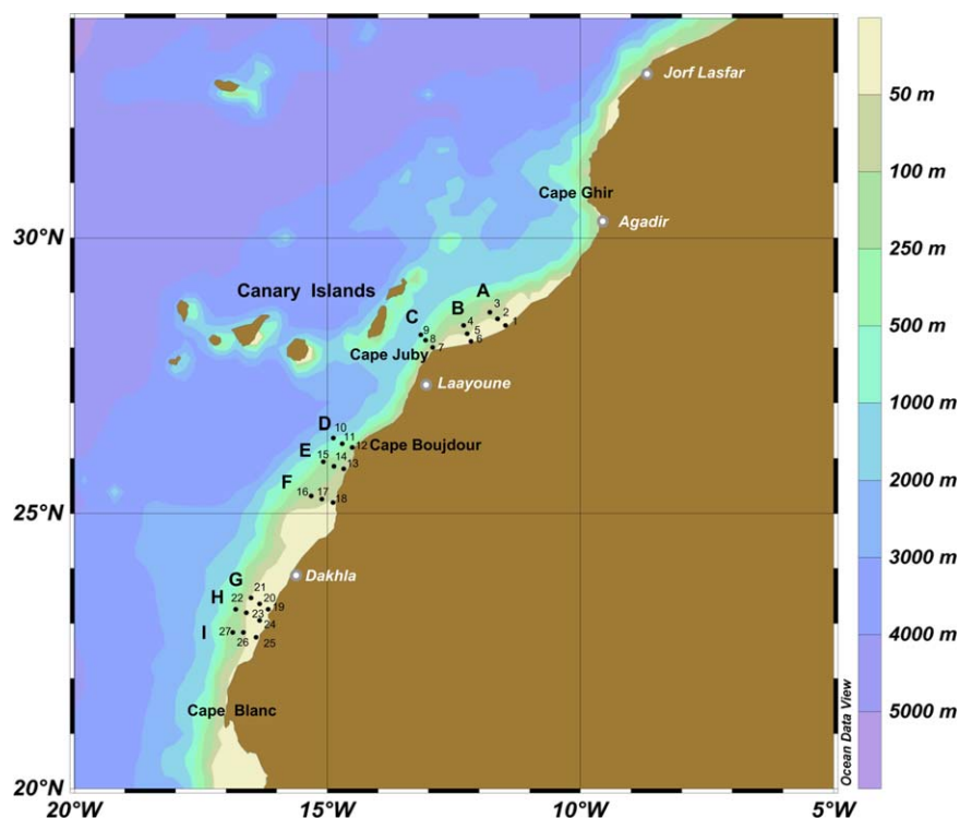
Figure 1. Map of stations (black dots and numbers) where total dissolvable and particulate samples were collected during the EPURE 2 cruise aboard the R/V Antea. Transect definitions are indicated by capital letters.
