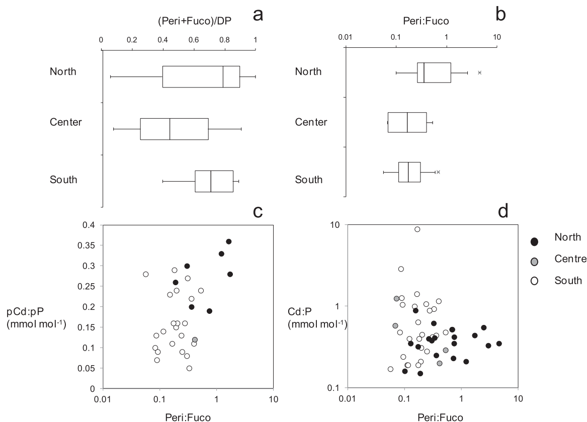
Figure 8. (a) Box plot representation of the (peridinin + fucoxanthin) over the various diagnostic pigments (DP, defined by Vidussi et al. [2001] as the sum of: zeaxanthin + chlorophyll b + alloxanthin + 19'-hexanoyloxyfucoxanthin + 19' - butanoyloxyfucoxanthin + fucoxanthin + peridinin) for showing the importance of the microphytoplanktonic pool in the various areas; (b) box plot representation of the peridinin: fucoxanthin ratio for showing the dominance of dinoflagellates (high ratio) or diatoms (low ratio); (c) pCd:pP ratio ( \text{mmol mol}^{-1} ) over Peridinin:fucoxanthin ratio and (d) Cd:P ratio ( \text{mmol mol}^{-1} ) over Peridinin:fucoxanthin ratio for the northern (black circles), central (grey circles), and southern areas (white circles).
