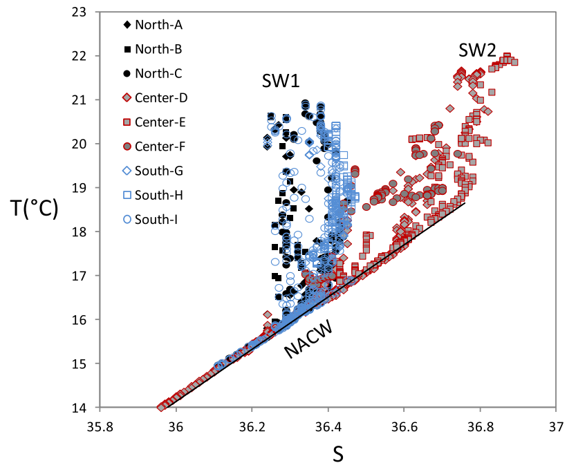
Figure 3. T-S diagrams at the various sections for the northern (black), central (red), and southern (blue) areas. The black line indicates the typical T-S relationship of the North Atlantic Central Waters [Tomczak, 1981; Knoll et al., 2002]. SW1 and SW2 correspond to different superficial water types.
