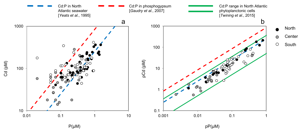
Figure 6. (a) Cd (pM) over P ( \mu\text{M} ) and (b) pCd (pM) over pP ( \mu\text{M} ) in the studied system. Black, grey, and white circles indicate samples collected in the northern, central, and southern areas, respectively. Blue dashed line indicates the Cd:P ratio reported in North Atlantic seawater [Yeats et al. , 1995]. Red dashed line indicates the Cd:P ratio in phosphogypsum [Gaudry et al. , 2007]. Green lines indicate the Cd: P range reported in phytoplankton cells of the North Atlantic [Twining et al. , 2015].
