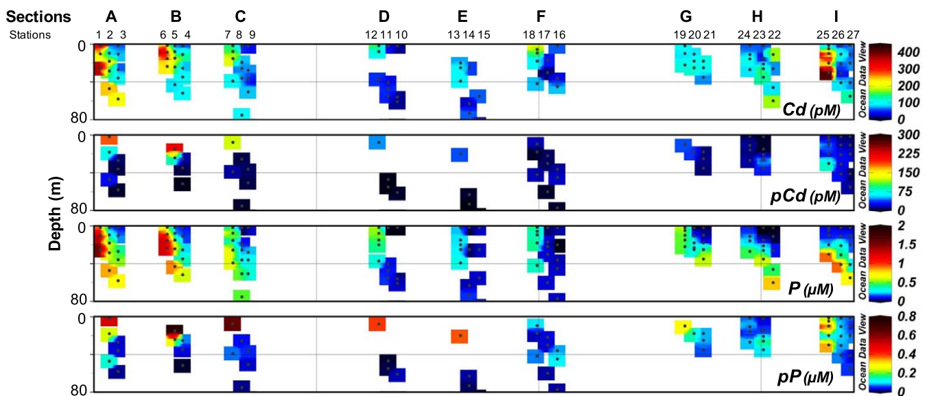
Figure 4. Vertical distributions of Cd (total dissolvable Cd, pM), pCd (particulate Cd, pM), P (Soluble Reactive Phosphorus, µM), and pP (particulate P, µM) along the nine sections (A to I). For each section, the inshore station is displayed on the left.
