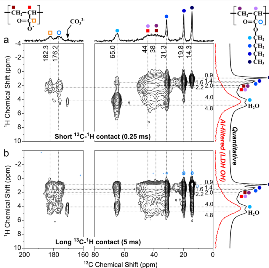
Figure 7: Solid-state ^{13}\text{C}\{^1\text{H}\} HETCOR NMR spectra of \text{MgAl-}P(\text{AA}_{8.5}\text{-}staf\text{-BA}_{8.5})\text{-CTPPA} , and collected at: a) short CP contact time (0.25 ms) to emphasize short ^1\text{H}\text{-}^{13}\text{C} proximities (primarily C–H bonds) and b) at long CP contact time (5 ms) to allow magnetization transfer across longer ^1\text{H}\text{-}^{13}\text{C} distances. The 1D spectrum on the top is the quantitative ^{13}\text{C} echo-MAS spectrum. 1D ^1\text{H} spectra on the right were collected at fast (60 kHz) MAS to reduce broadening due to ^1\text{H}\text{-}^1\text{H} interactions: the black spectrum is a quantitative ^1\text{H} echo-MAS and the red corresponds to a ^1\text{H}\{^{27}\text{Al}\} CP-MAS experiment selectively probing the LDH OH protons in close proximity to the framework Al sites.
