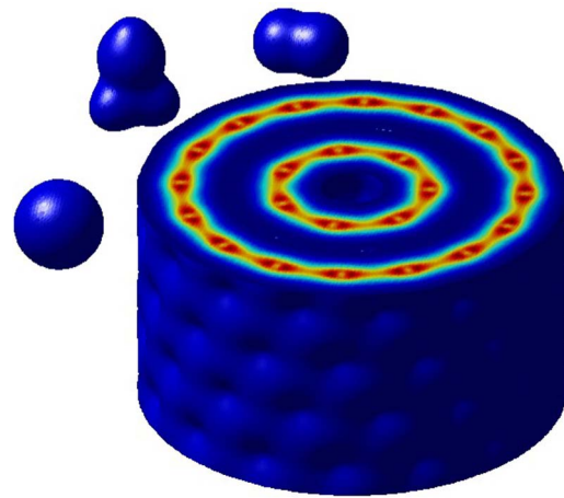
FIG. 4. (Color online) Electronic density at a van der Waals radius for Ar, methanol, \text{O}_2 , and DWCNT. The CNT surface is not uniform.
