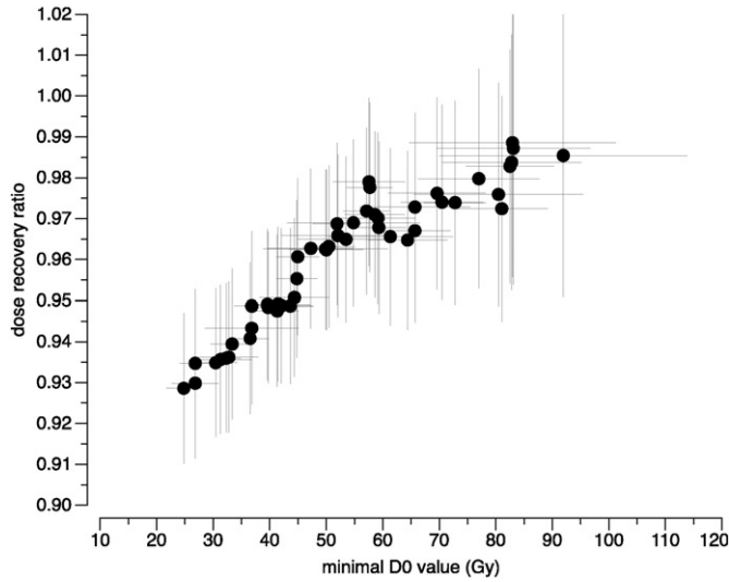
Fig. 6. Dose recovery ratio against minimal D_0 value of the grains used for the computation of the central recovered dose (Galbraith et al., 1999), sample T14, single-grain mode. The dose to recover was 70 Gy. It can be observed that for this sample, while the dose recovery ratio for the whole distribution is already within the [0.9;1.1] interval, it is significantly improved with D_0 thresholding.
