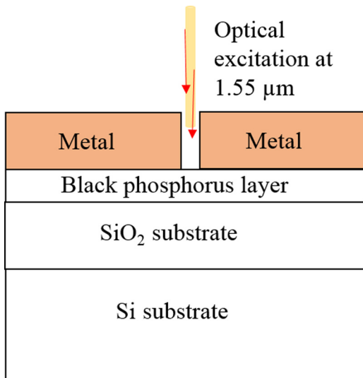
FIG. 1. Schematic diagram of the black phosphorus microwave photoconductive switch.
