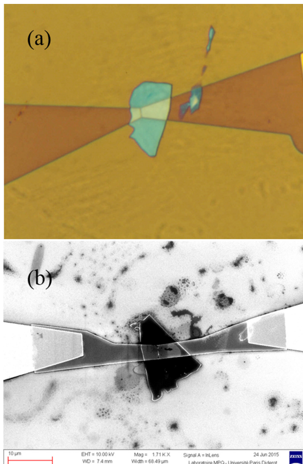
FIG. 2. (a) Optical image of an exfoliated black phosphorus layer in blue with two electrodes, before the evaporation of palladium. The electrode gap length is 100 nm. (b) Scanning electron microscope image of a black phosphorus based photoconductive switch. The exfoliated layer is in black, the two palladium electrodes in grey, and the gold waveguide in white.
