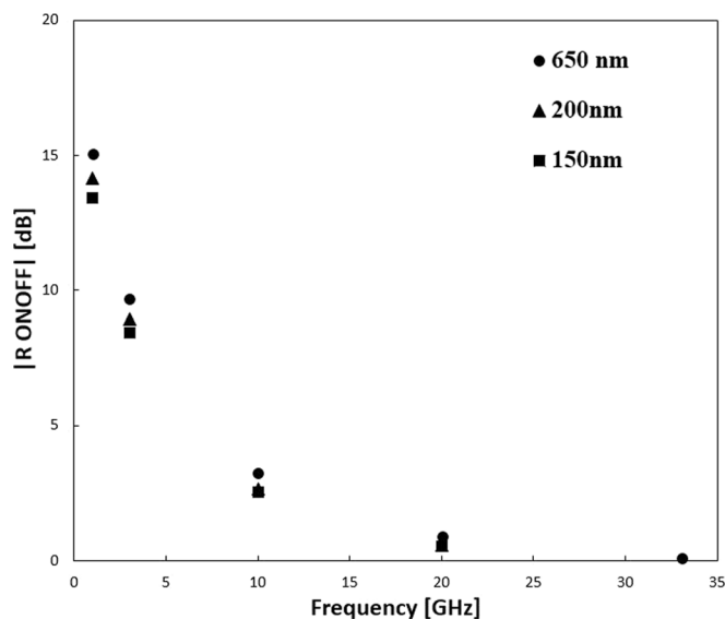
FIG. 6. Plot of the ON/OFF ratio of the silicium substrate based microwave photoconductive switches with electrode gaps of 150 nm, 200 nm, and 650 nm, for a laser power of 25.6 mW and a wavelength of 1.55 \mu\text{m} .
