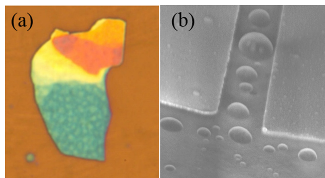
FIG. 3. Effects of the extreme sensitivity of the exfoliated bP to the environment. (a) Optical image of a bP flake several hours after exfoliation. Apparition of droplets at the surface. (b) Scanning electron microscope image of the surface of a black phosphorus layer at especially the gap between the two palladium electrodes one hour after exfoliation. Apparition of droplets at the surface of the black phosphorus.
