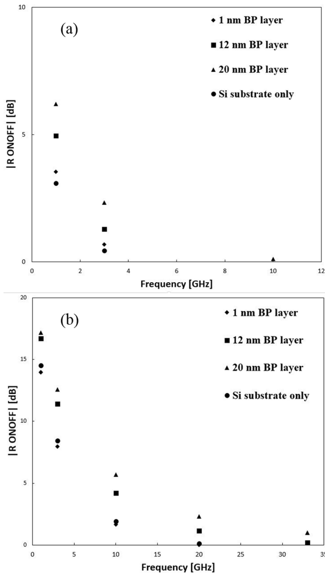
FIG. 4. Plot of the ON/OFF ratio of the black phosphorus based microwave photoconductive switches with a black phosphorus layers thickness of 1 nm, 12 nm, and 20 nm, and the ON/OFF ratio of a switch without black phosphorus (based on Si/SiO 2 substrate) versus frequency, (a) for a laser power of 20 mW and a wavelength of 1.55 μm and (b) for a laser power of 50 mW and a wavelength of 1.55 μm.
