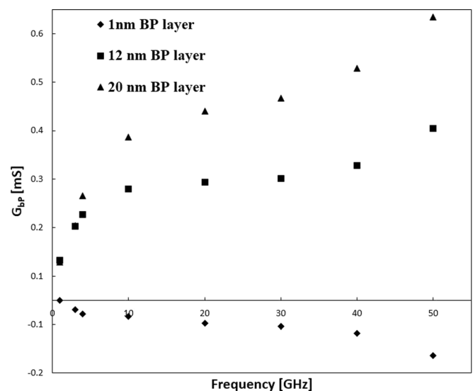
FIG. 5. Plot of the conductance of the BP based photoconductive switch with different layer thicknesses, for a laser power of 50 mW and a wavelength of 1.55 μm.
