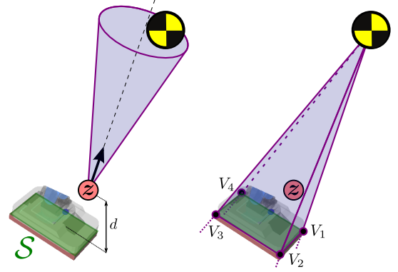
Fig. 1. The two necessary and sufficient conditions for contact stability of the Floating-base Inverted Pendulum. Friction (left): the COM belongs to the contact friction cone C projected from the ZMP z . Center of pressure (right): the ZMP z belongs to the cone projected from the COM and containing the vertices of the contact surface S .
