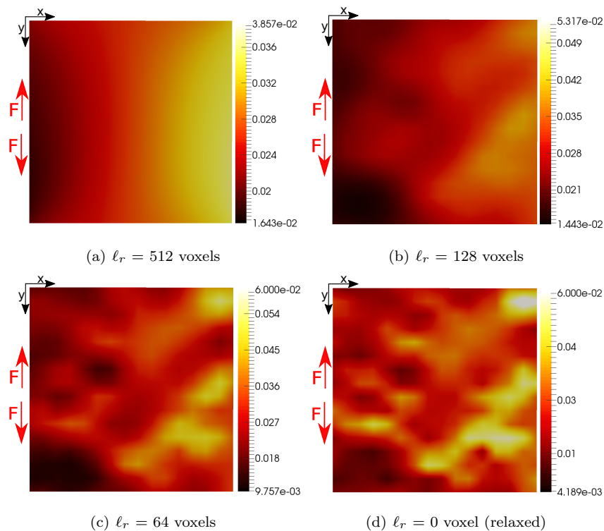
Fig. 11 Equivalent strain maps of mid-thickness section for the first loading step and four different regularization lengths
