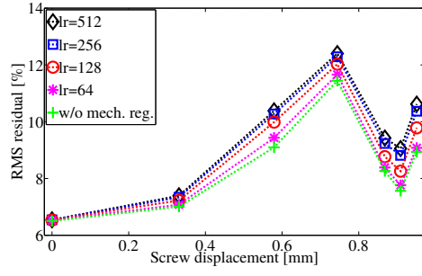
Fig. 9 Root mean square gray level residual (normalized by dynamic range of the volume - 256 gray levels) for various regularization lengths (expressed in voxels)
