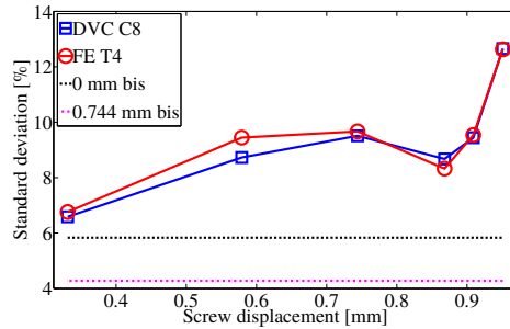
Fig. 24 Standard deviation for the dimensionless gray level residual fields for all loading steps (FE results obtained with h_2 mesh)
