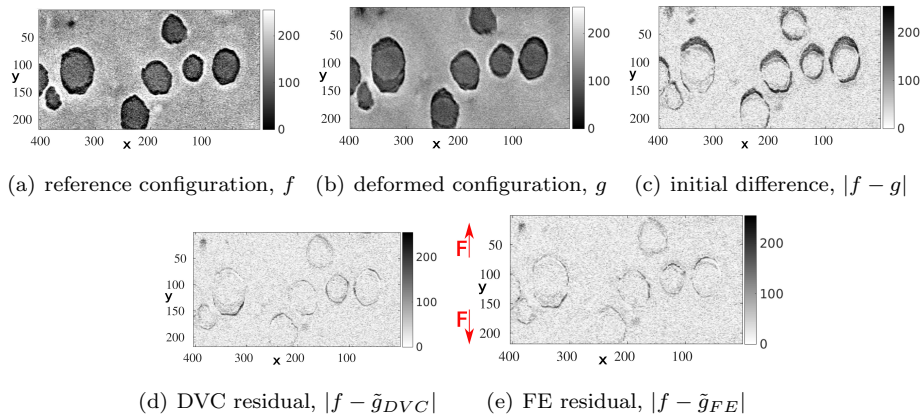
Fig. 23 Microstructure section in the (a) reference and (b) deformed states. Absolute gray level differences between the two initial states (c) and after correction with DVC (d) and FE (e) displacements (obtained on h_2 mesh) for third loading step
