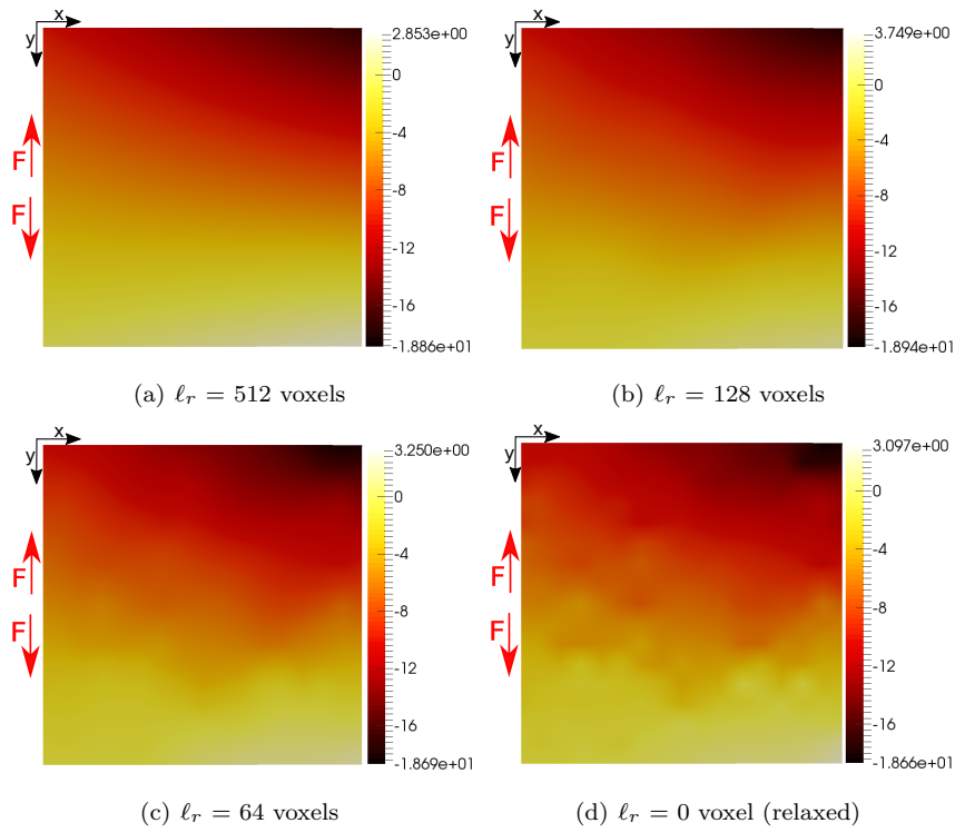
Fig. 10 Displacement fields of mid-thickness section for the first loading step and four different regularization lengths
