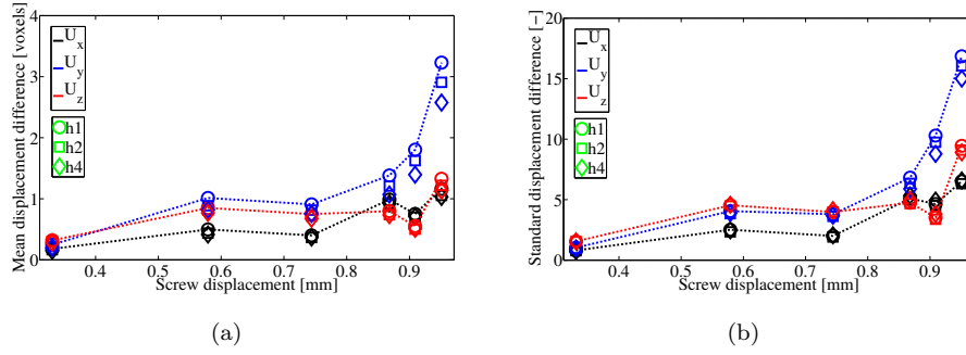
Fig. 22 (a) Mean values and (b) standard deviations of the difference between the measured and simulated displacement fields for different FE mesh sizes. Standard deviations are normalized by the corresponding DVC uncertainties
