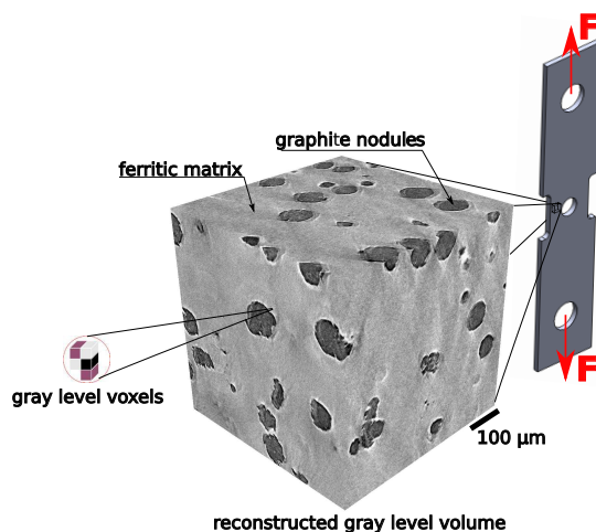
Fig. 3 Reconstructed volume as a spatial discrete matrix of gray level values
