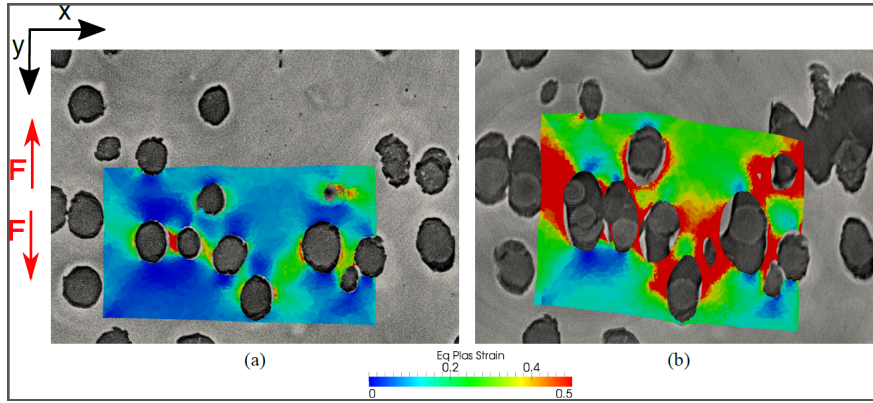
Fig. 18 Equivalent plastic strain obtained by the FE simulation superimposed with experimental images at a macroscopic displacement of: (a) 578 \mu\text{m} , (b) 910 \mu\text{m}
