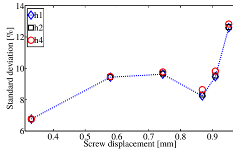
Fig. 25 Standard deviation gray level residuals for all loading steps with three different FE discretizations
