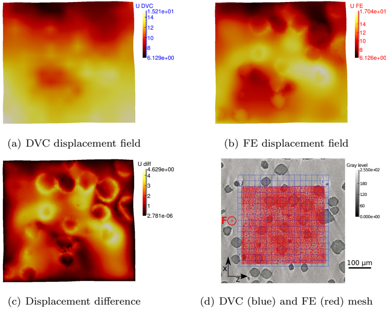
Fig. 20 Section normal to y -direction: (a) DVC displacement field magnitude, (b) FE displacement field magnitude, (c) absolute difference between them and (d) DVC and FE meshes for the third loading step. All reported values are expressed in voxels (1 voxel \leftrightarrow 1.1 \mu\text{m} ) and correspond to the FE mesh h_2
