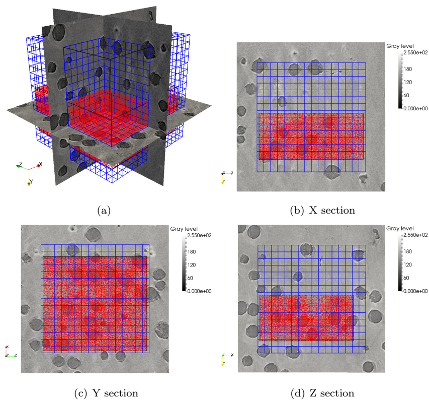
Fig. 19 (a) DVC (blue) and FE (red) meshes plotted over the corresponding cast iron microstructure in (a) isometric view and (b-d) sections normal to X , Y and Z axes
