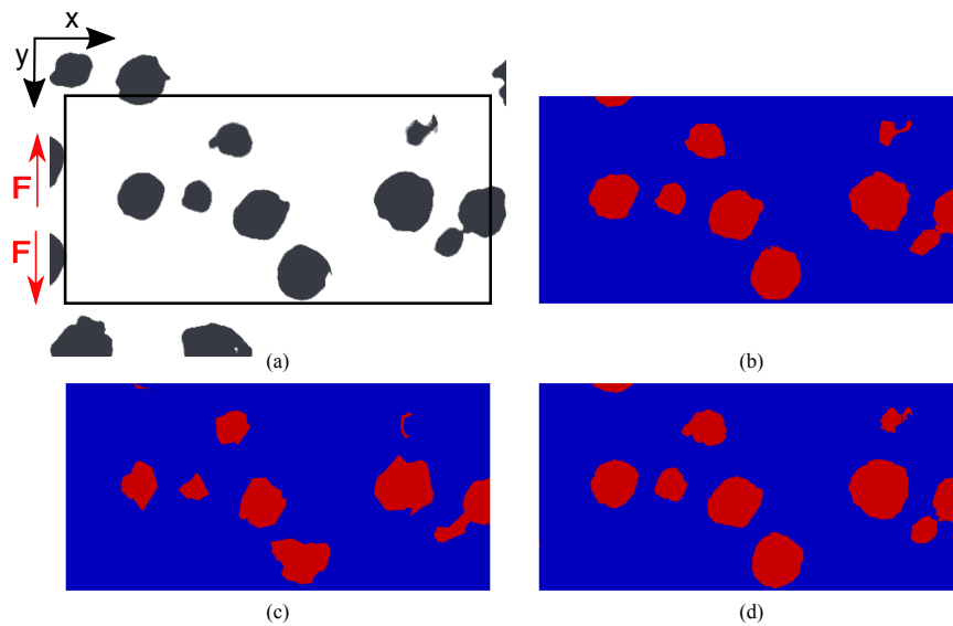
Fig. 14 Matrix and nodules at midsection of: (a) the image, (b) the reference mesh h2 , (c) the coarse mesh h4 , (d) the fine mesh h1
