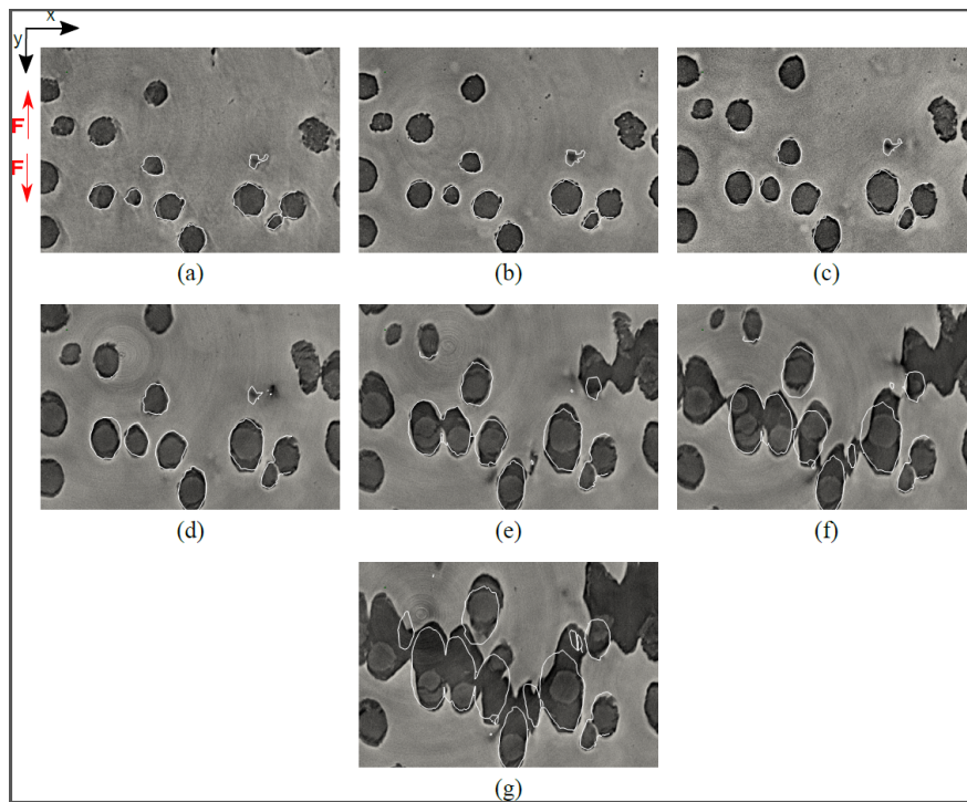
Fig. 17 Comparison between the void/matrix interface obtained by the FE simulation (thin white line) and the experimental images at a macroscopic displacement of: (a) 0 \mu\text{m} , (b) 330 \mu\text{m} , (c) 578 \mu\text{m} , (d) 744 \mu\text{m} , (e) 868 \mu\text{m} , (f) 910 \mu\text{m} , (g) 950 \mu\text{m}
