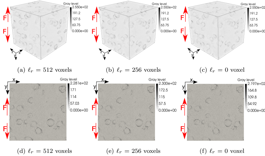
Fig. 8 (a)-(c) Isometric view of the gray level residual field and (d)-(f) through thickness section with the residual map for first loading step and three different regularization lengths
