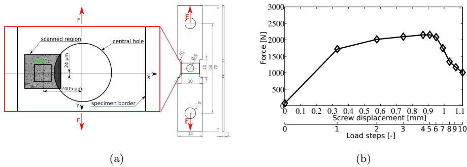
Fig. 2 (a) Schematic view of the sample with the scanned region close to the central hole. Section of the reconstructed volume with the position of the region of interest. (b) Macroscale force-displacement curve
