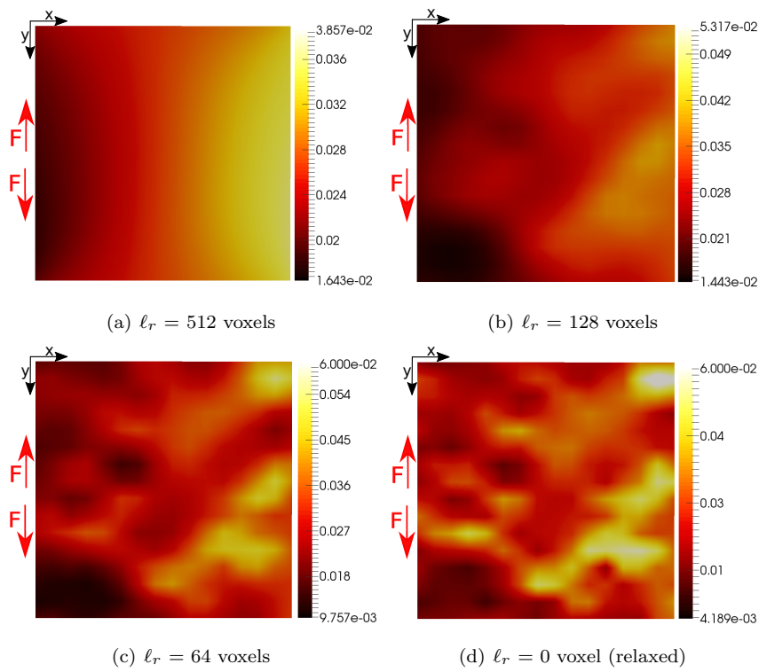
Fig. 11 Equivalent strain maps of mid-thickness section for the first loading step and four different regularization lengths
