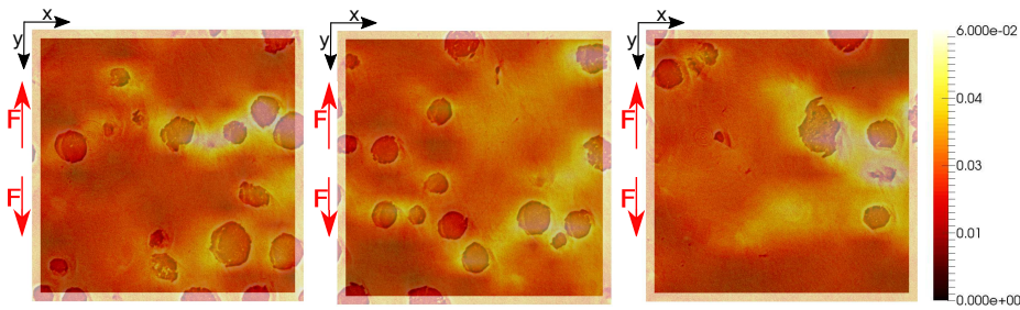
Fig. 12 Equivalent strain maps plotted together with the corresponding microstructure sections for the first loading step (unregularized DVC) and different positions along the thickness direction
