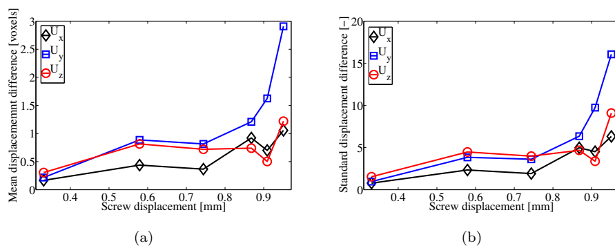
Fig. 21 (a) Mean values and (b) standard deviations of the difference between the measured simulated displacement fields for the FE mesh h_2 . Standard deviations are normalized by the corresponding DVC uncertainties
