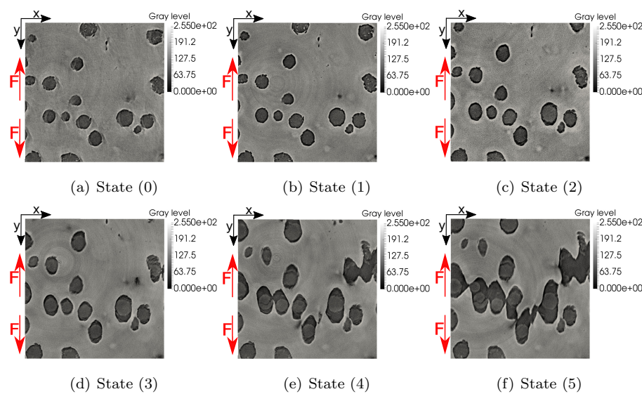
Fig. 7 Through thickness section showing nodules embedded in the matrix for the undeformed state (a) and after the first five loading steps (b)-(f)
