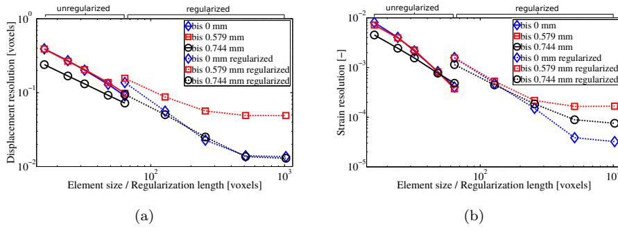
Fig. 6 Standard displacement (a) and equivalent strain (b) resolutions as functions of the element size or regularization length
