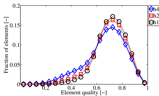
Fig. 15 Distribution of mesh quality at the initial state for the three tested mesh settings
