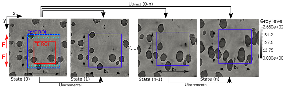
Fig. 5 Difference between incremental and direct DVC procedures
