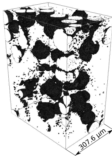
Fig. 4 3D rendering of all dark features of the nodular cast iron reconstructed volume
