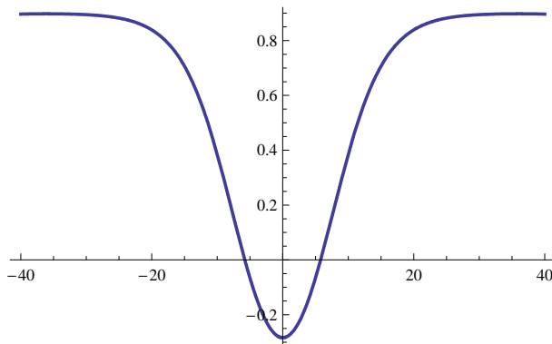
Fig. 2 Pulse (in form \rho = \mathcal{F}_1(x) ) near the water critical point at T \simeq 646^\circ\text{K} when \gamma = 0 (second-gradient model); x -axis unit is 2.7 \times 10^{-7} cm \equiv 2.7 nm and y -axis unit is 3.2 \times 10^{-6} g/cm 3 .
