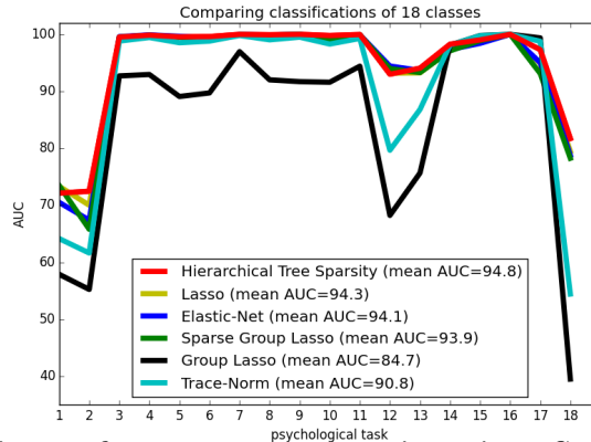
Fig. 3. Prediction performance across sparsity priors. Comparing the performance of logistic regression estimators with 6 different structured and unstructured sparse regularization penalties ( colors ) in classifying neural activity from 18 psychological tasks (cf. 7, Table 1). The area under the curve (AUC) is provided on an identical test set as class-wise measure ( y-axis ) and across-class mean ( legend ). Simultaneous knowledge of both region and network neighborhoods was hence most beneficial for predicting tasks from neural activity.
