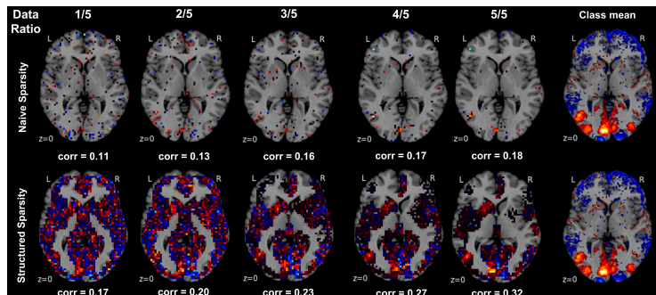
Fig. 4. Sample complexity in naive versus informed sparse model selection. Ordinary \ell_1 -penalized logistic regression ( upper row ) is compared to hierarchical-tree-penalized logistic regression ( \alpha = 1, \beta = 1 , lower row ) with increasing fraction of the available training data to be fitted ( left to right columns ). For one example (i.e., “View tools”) from 18 psychological tasks (cf. 7, Table 1), unthresholded axial maps of recovered model weights are quantitatively compared against the sample average of that class ( rightmost column , thresholded at the 75 th percentile). This notion of weight recovery was computed by Pearson correlation ( corr ). In the data-scarce scenario, ubiquitous in neuroimaging, hierarchical tree sparsity achieves much better support recovery. In the data-rich scenario, biologically informed logistic regression profits more from the available information quantities than biologically naive logistic regression.
