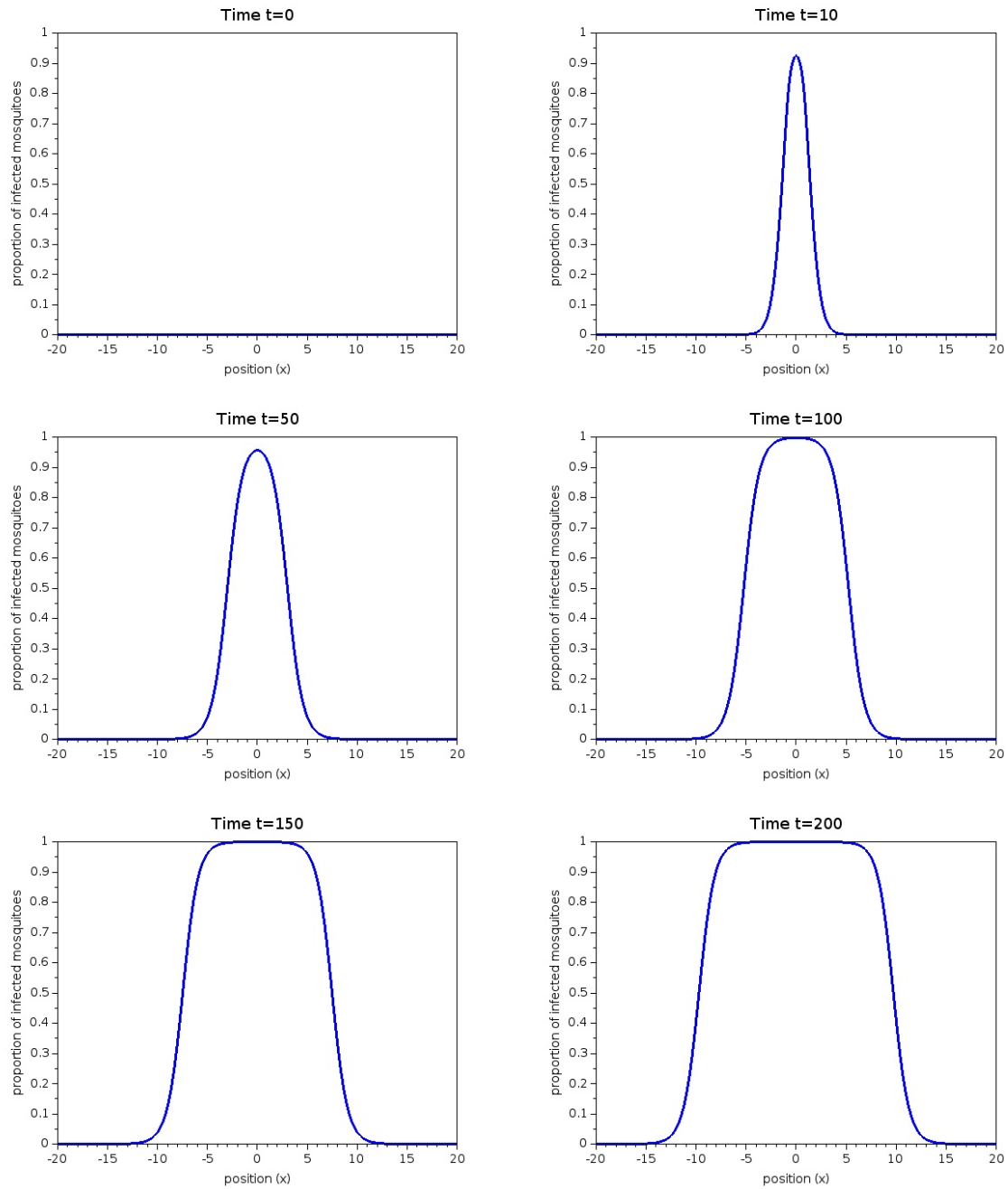
Figure 1: Time dynamics of the proportion of infected population with a feedback control function as in system (16). From top left to bottom right, the plotted times are : initial time, t=10 , t=50 , t=100 , t=150 , t=200 .
