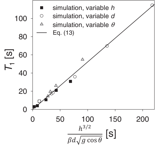
FIG. 6. Scaling of T_1 , the characteristic acceleration time scale, with flow thickness h , average grain size d , and inclination angle \theta . Points are simulation results for systems with h = 12d-96d , d = 0.1 m, and \theta = 17^\circ (squares); h = 48d, 70d , or 96d , d = 0.1-1 m, and \theta = 17^\circ (circles); and h = 48d , d = 0.1 or 1 m, and \theta = 18^\circ-25^\circ (triangles). The solid line is the analytical prediction (13).
