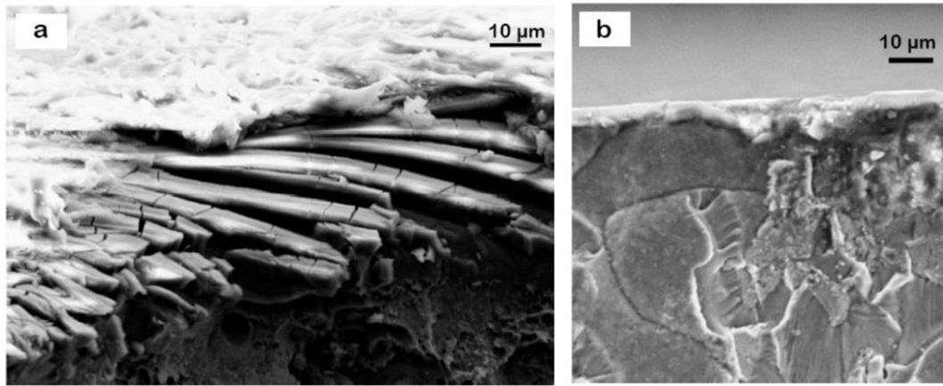
Fig. 19. SEM observations of anodic films after corrosion fatigue tests in 0.85 M NaCl at 80% of YSO_2 of a) hydrothermally sealed material and b) (B1 + B2) sealed material.
