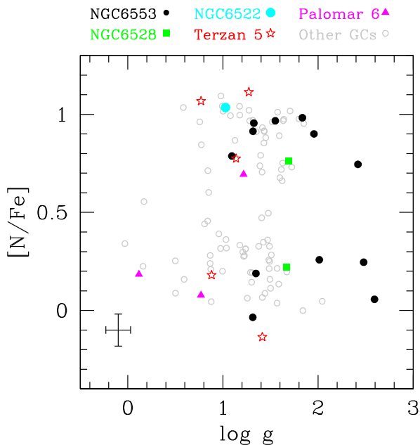
Figure 2. Nitrogen abundance ratios as a function of surface gravity for the sample stars. Stars of approximately the same gravity (thus same evolutionary stage) have vastly different [N/Fe], which cannot be explained by mixing.
