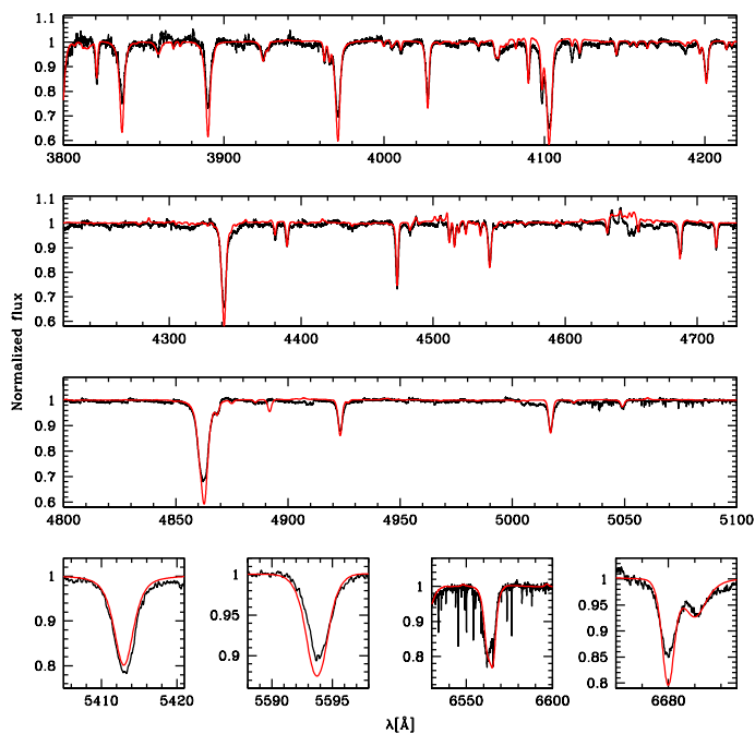
Fig. B.9. Best fit (red) of the observed spectrum (black) of HD 162978.
