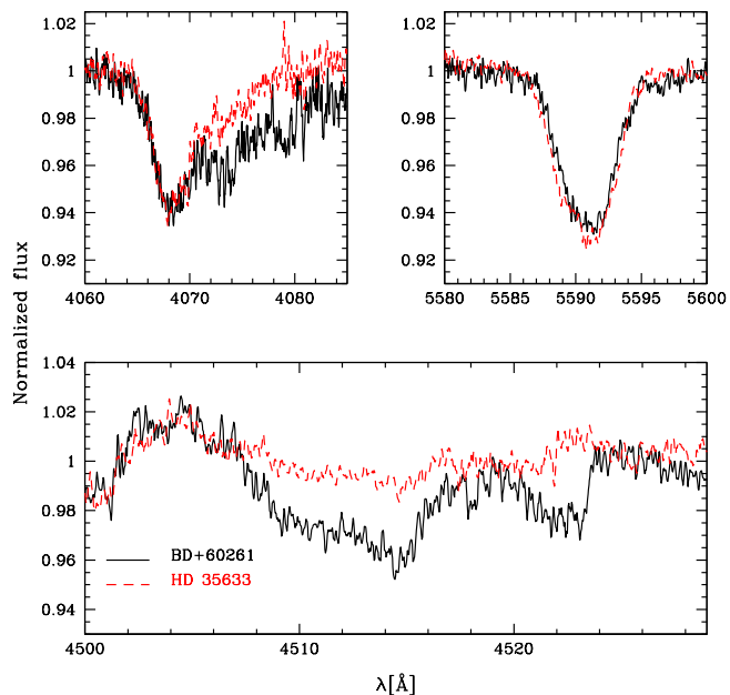
Fig. 5. Comparison between the observed spectrum of BD +60261 (black solid line) and HD 35633 (red dashed line). C III 4070, O III 5592 and the N III lines around 4510 \text{ Å} are displayed in the upper left, upper right and bottom panel respectively. Both stars have very similar V \sin i .
