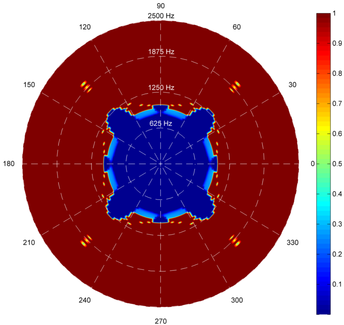
Figure 17. Directivity diagram of the Cneg fully shunted lattice. Distance from the center is frequency. Color is Ind (blue: some waves can propagate in the lattice, red: band gap).
