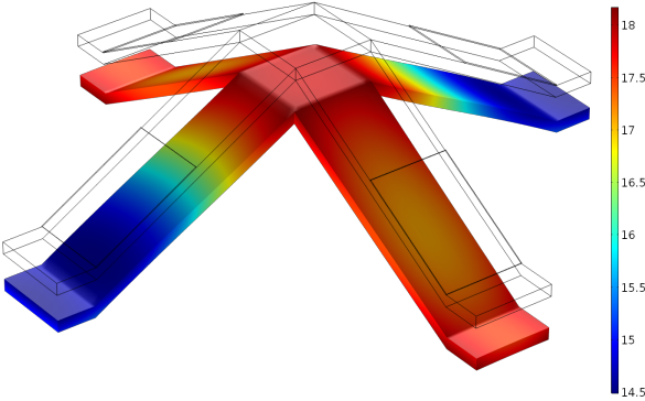
Figure 6. Shape of mode occurring at 110 Hz, with \text{Real}(k_n) \approx 0.7723 \frac{\pi}{L} , corresponding to red square in figure 5. Color scale corresponds to modal kinetic energy density. Grey lines show the undeformed cell.
