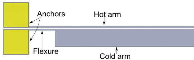
Figure 1. U-shaped electrothermal microractuator.
