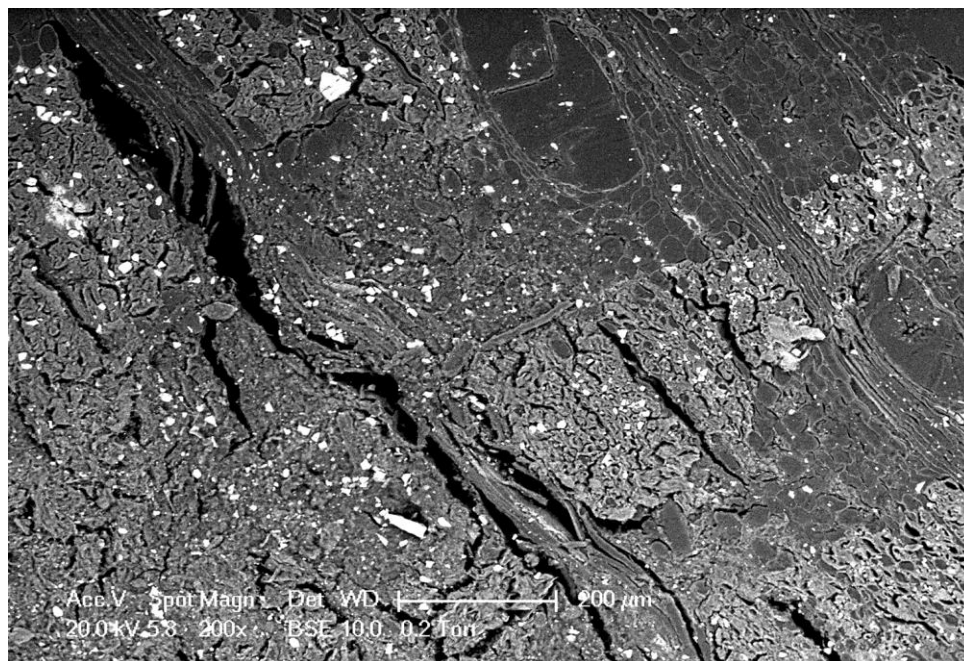
Figure 4: SEM micrographs showing the characteristic cell shape of sound vessels and fibers, as well the deformation of the wood as result of natural aging.
