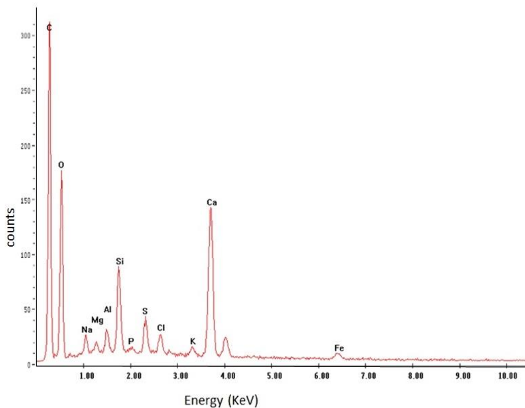
Figure 12: SEM/EDS pattern of black pigment.
