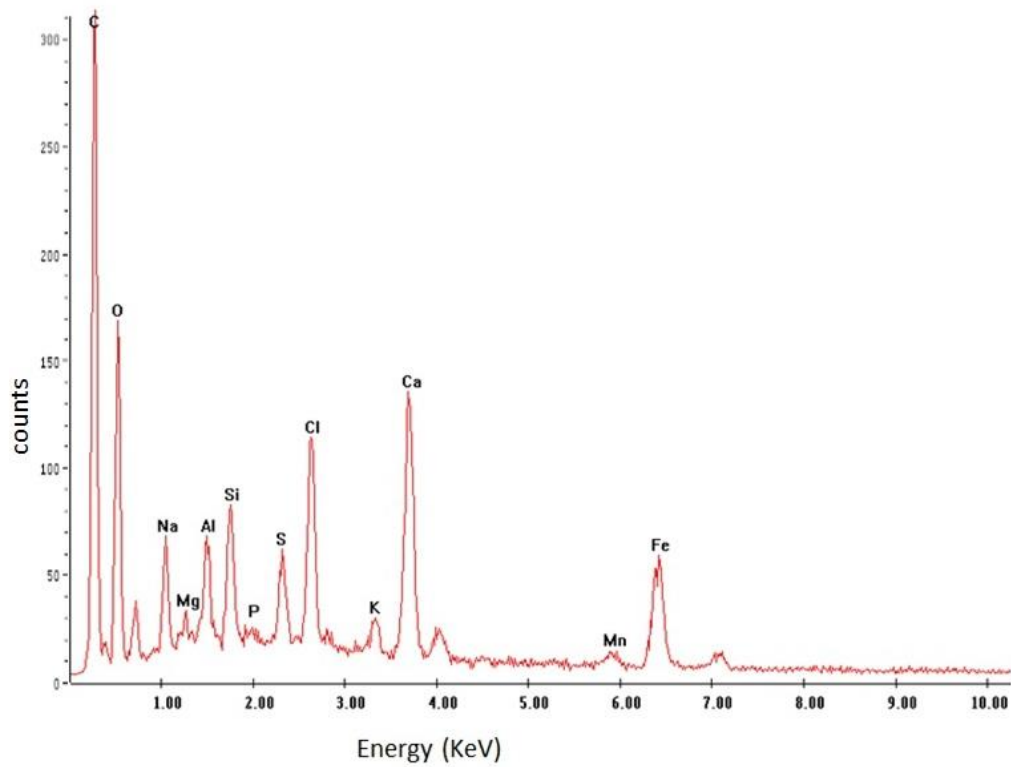
Figure 13: SEM/EDS pattern of red pigment.
