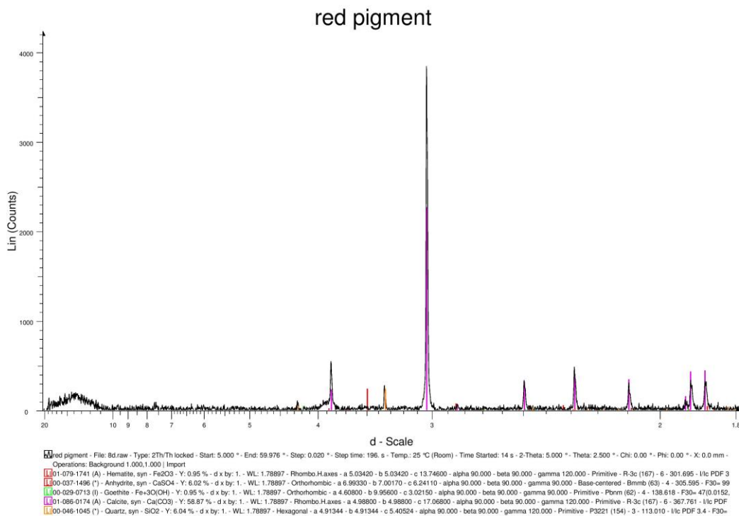
Figure 14: XRD pattern of red pigment.
