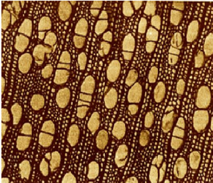
Figure 3: Optical microscope photo of section confirming that the type of the wood is Salix sp. (willow).
