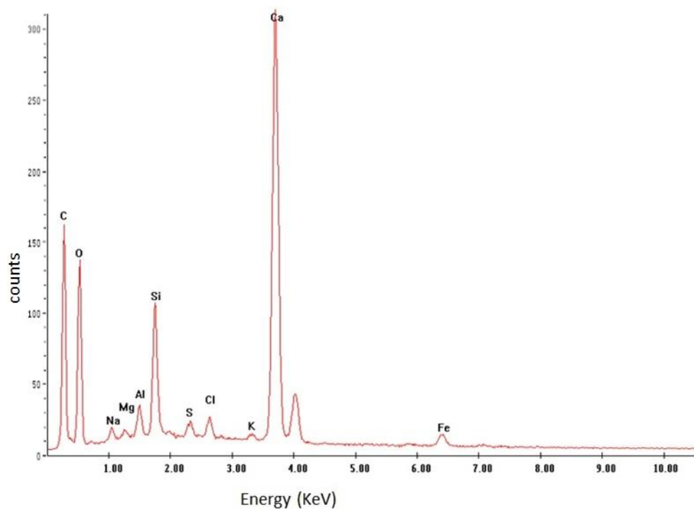
Figure 11: Pattern showing the analysis of the ground layer and the high proportion of calcium.
