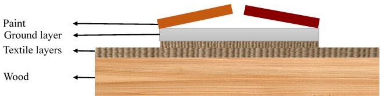
Figure 2: The structure of the consecration panel.
