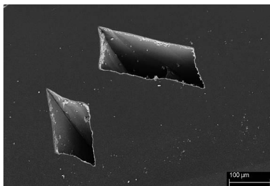
Fig. 4: Close view by SEM of the channel openings of sample MSC19. Notice the sharp concave shapes. The inner walls are smooth (even at a 10 time higher magnification). Notice the crack at the crossing of two inner walls (forming acute angle).
