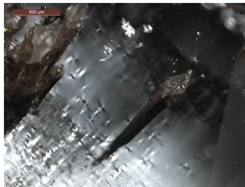
Fig. 3: Photomicrograph of a channel under crossed (linear) polarizers of sample MSC67. There is less to no abnormal birefringence next to the channels, while the rest of the diamond is strained (especially around the disk-crack-like defects).
