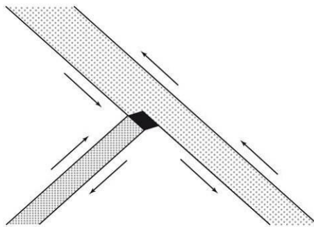
Fig. 6: When two twin lamellae meet, a hollow channel called Rose channel may appear (redrawn from [35]).
