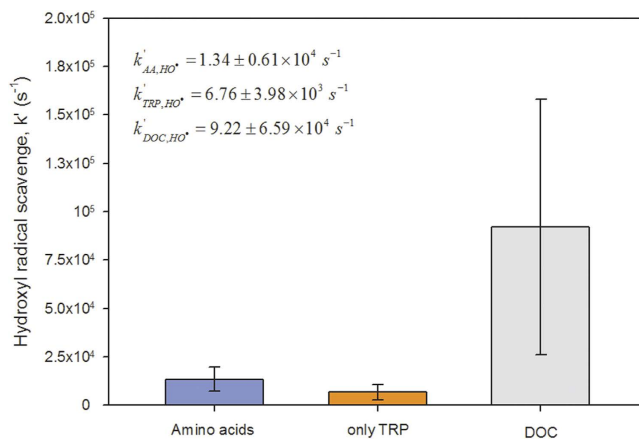
Figure 4. HO^{\bullet} scavenging rates ( k' ) of AAs, TRP and DOC. These values were determined based on the average values of \sum_i k_{HO^{\bullet},AA}^{II} [AA]_i , k_{HO^{\bullet},TRP}^{II} [TRP] and k_{HO^{\bullet},DOC}^{II} [DOC] using the concentrations and second-order rate constants reported in Tables S1 and S3. The k_{HO^{\bullet},DOC}^{II} value was taken from Arakaki et al. 39 .
