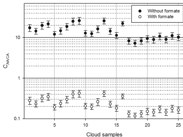
Figure 3. Ratio of the scavenging rate constants of HO• (expressed in s -1 ) with AAs and short-chain CAs (C AA/CA ) without (filled circles) and with (empty circles) formate (calculated using equation 1). The error bars were determined by considering the uncertainties associated with AA quantification in each sample.
