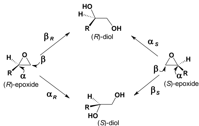
Figure 2. Attack at the oxirane ring can occur at either the terminal carbon atom, which results in a diol product with retained configuration ( \beta -attack), or the carbon atom with the substituent R, resulting in a diol with an inverted configuration ( \alpha -attack). The percentages of epoxide molecules following a particular reaction pathway are represented by the corresponding regioselectivity coefficients; the following relationships between the four regioselectivity coefficients are valid: \alpha_R + \beta_R = 100\% , and \alpha_S + \beta_S = 100\% .
