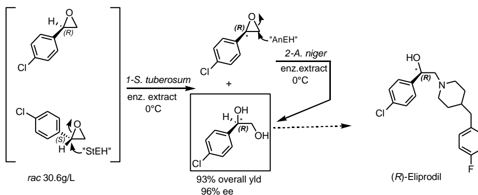
Figure 8. Enantioconvergent bihydrolytic transformation of para -chlorostyrene oxide using a bi-enzymatic process. The sequential use of Solanum tuberosum and Aspergillus niger EHs as biocatalysts led to the formation of enantiopure ( R )- para -chlorophenyl-1,2-diol, a chiral building block for the synthesis of ( R )-Eliprodil.
