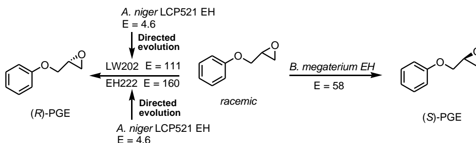
Figure 19. Biohydrolytic kinetic resolutions of racemic-PGE. Use of enantiocomplementary wild-type and evolved mutant EHs for the preparation of two antipodes of PGE.
