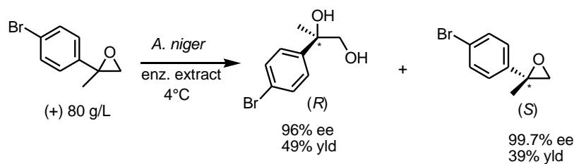
Figure 12. Kinetic hydrolytic resolution at high substrate concentration of para -bromo- \alpha -methyl styrene oxide using an enzymatic extract of A. niger .
