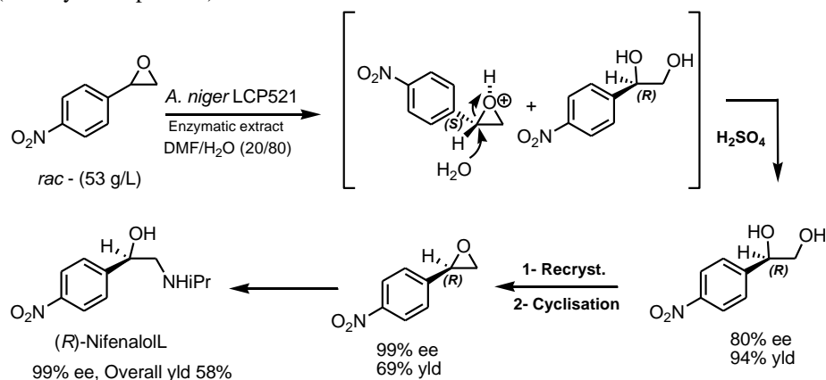
Figure 9. Enantioconvergent synthesis of the \beta -blocker ( R )-Nifenalol using a combined chemoenzymatic approach.
