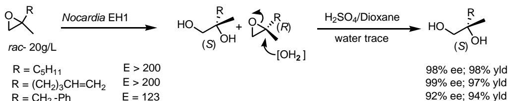
Figure 20. Chemoenzymatic deracemization of rac-gem -disubstituted oxiranes.
