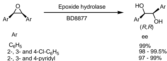
Figure 28. Desymmetrization of aryl meso -epoxides with BD887 obtained from DNA libraries of environmental samples.
