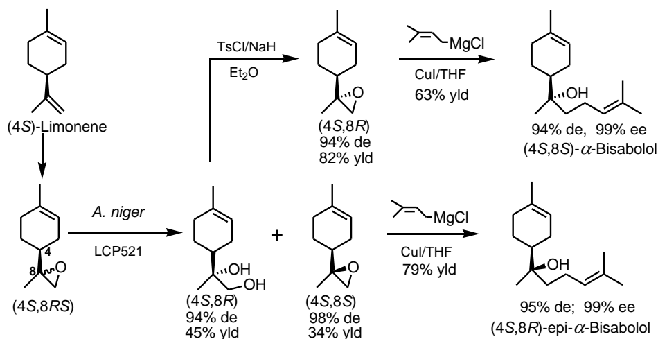
Figure 43. Diastereoselective biohydrolysis of (4 S ,8 RS )-limonene oxide using whole cells of the strain A. niger LCP521 as biocatalyst, leading to the synthesis of \alpha -Bisabolols.
