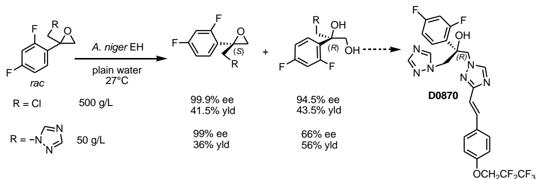
Figure 31. Preparative hydrolytic resolution of rac -1-chloro- and 1- triazole-2(2,4-difluorophenyl)-2,3-epoxypropane using AnEH as biocatalyst. The latter compound is a useful building block for the synthesis of enantiopure D0870.
