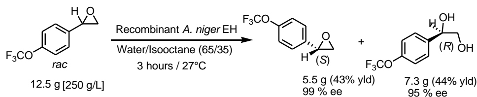
Figure 10. Preparative scale synthesis of enantiopure (4-trifluoromethoxyphenyl)-oxirane using a partially purified recombinant EH from Aspergillus niger LCP521 as a biocatalyst.
