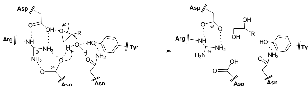
Figure 5. Proposed catalytic mechanism of the limonene-1,2-epoxide hydrolase from Rhodococcus erythropolis and the EH from Mycobacterium tuberculosis . The catalytic water molecule is activated by the formation of hydrogen bonds involving aspartic acid, arginine and tyrosine residues. At the same time, polarization and activation of the oxirane ring is achieved by hydrogen bonding with the oxirane oxygen involving another aspartic acid residue.
