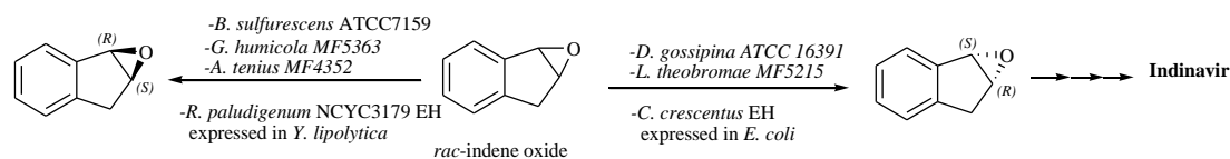
Figure 17. Biohydrolytic kinetic resolution of racemic indene oxide. Access to (1 S ,2 R )- or (1 R ,2 S )-indene oxide as a function of the biocatalyst used.
