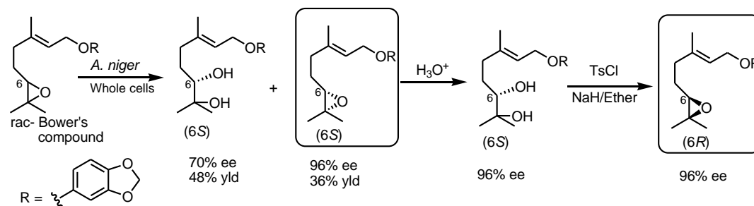
Figure 24. Synthesis of both enantiomers of Bower's compound using whole cells of the fungus A. niger LCP521 as biocatalyst.
