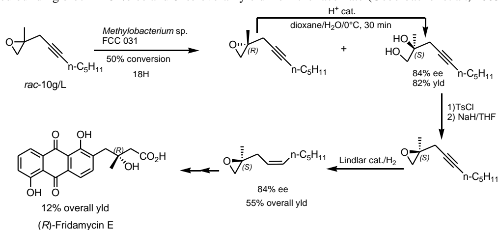
Figure 51. Asymmetric total synthesis of (R)-Fridamycin E.
