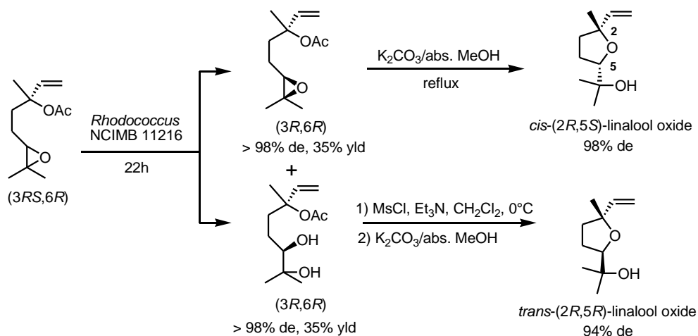
Figure 42. Chemo-enzymatic synthesis of cis - and trans -Linalool oxide using bacterial EH.
