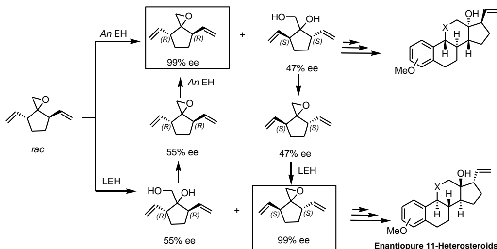
Figure 22. Preparative hydrolytic resolution of trans -divinylspiroepoxide using AnEH and LEH as biocatalysts allowing the synthesis of enantiopure 11-heterosteroids.
