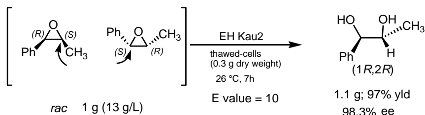
Figure 16. Preparative enantioconvergent biohydrolysis of racemic cis - \beta -methylstyrene oxide using the EH Kau2.
