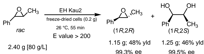
Figure 15. Preparative-scale kinetic resolution of racemic trans - \beta -methylstyrene oxide using the EH Kau2 at high substrate concentration.
