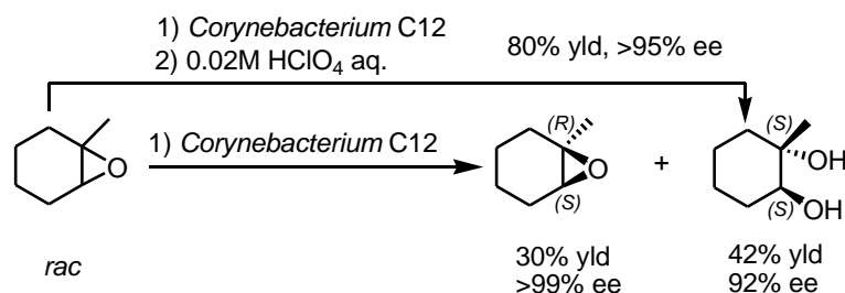
Figure 25. Chemoenzymic resolution and deracemisation of rac -1-methyl-1,2-epoxycyclohexane using whole cells of Corynebacterium C12.
