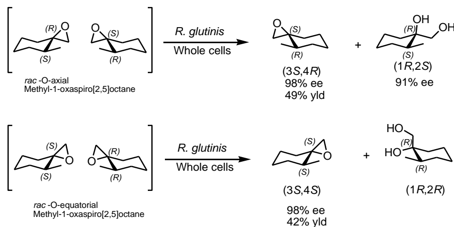
Figure 21. Kinetic resolution of O-axial or O-equatorial 4-methyl-1-oxaspiro[2,5]octane by Rhodotorula glutinis EH.
