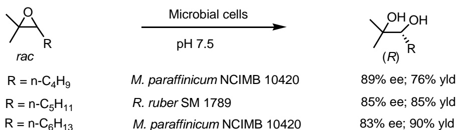
Figure 26. Deracemization of three rac -trialkyl oxiranes via enantioconvergent biohydrolysis using whole cells of Mycobacterium paraffinicum and Rhodococcus ruber .
