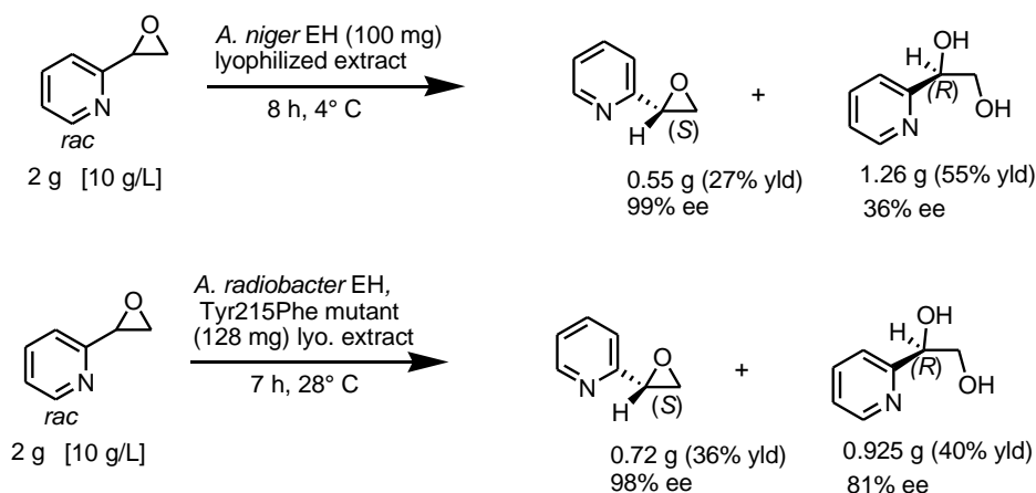
Figure 11. Preparative kinetic resolution of 2-pyridyloxirane with EHs from A. niger and A. radiobacter AD1 (mutant Tyr215Phe).
