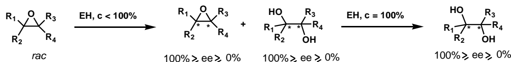
Figure 1. EH-catalyzed hydrolysis of a racemic epoxide, resulting in the formation of a vicinal diol with an enantiomeric excess of 100\% \geq ee_p \geq 0\% at complete conversion ( c = 100\% ) of the substrate. Depending on the EH-substrate interactions and consequently its substrate-related enantiomeric ratio or E-value (which depends on c and ee_s and characterizes the ability of the enzyme to discriminate between the two competing substrate enantiomers, Chen et al., 1982), enantiopure epoxide is obtained at a specific degree of conversion within the range of 50\% < c < 100\% . The kinetics of highly enantioselective EHs is characterized by a rapid hydrolysis of the preferred epoxide enantiomer, followed by a much slower hydrolysis of the remaining epoxide.
