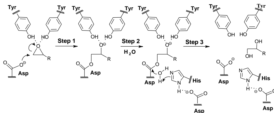
Figure 4. Proposed catalytic mechanism of EHs which are members of the \alpha/\beta -hydrolase fold superfamily.
