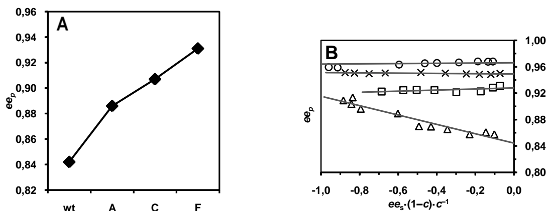
Figure 6. (A) Directed evolution of the metagenome-derived EH Kau2 towards an enantioconvergent biocatalyst. Five amino acid substitutions were sufficient to increase the degree of enantioconvergence from 84% ee_p for the wild-type EH (wt) to 93% ee_p for the final evolved variant (F), enabling the production of the R -diol with an ee -value of 93% at 28 °C in a complete conversion of racemic para -chlorostyrene oxide. A and C represent intermediate variants of the in vitro evolution process. Higher ee_p -values of up to 97% were determined in enantioconvergent reactions using lower temperatures (Kotik et al., 2013). (B) Determination of the regioselectivity coefficients \alpha_S and \alpha_R of the EH-catalyzed reaction using the wild-type and final evolved Kau2 variant with racemic para -chlorostyrene oxide as the substrate. Plotting ee_p against ee_s \cdot (1-c) \cdot c^{-1} enabled the determination of \alpha_R and subsequently \alpha_S as described in Kotik et al. (2010), using the intercept q and the slope m from the linear regression; for the calculations non-absolute values for ee_p and ee_s were used (see Moussou et al., 1998b). The following relationships are valid: \alpha_R + \beta_R = 1 , and \alpha_S + \beta_S = 1 . Wild-type EH at 28°C ( \Delta ): \alpha_R = 0.12 , \alpha_S = 0.95 ; final evolved variant at 28°C ( \square ): \alpha_R = 0.03 , \alpha_S = 0.96 ; at 18°C ( \times ): \alpha_R = 0.03 , \alpha_S = 0.98 ; at 8°C ( \circ ): \alpha_R = 0.02 , \alpha_S = 0.98 .
