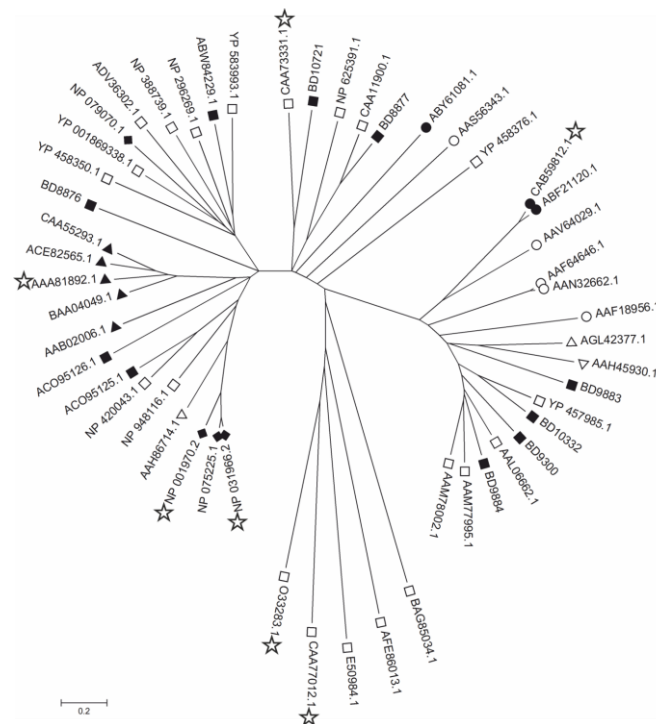
Figure 3. Phylogenetic relationships among protein sequences encoding EHs with confirmed activities. Each sequence is represented by its GenBank accession number; for sequences and further data regarding EHs with codes starting with BD, see Zhao et al. , 2004. The data set includes sequences of mammalian EHs (◆), plant EHs (▲), fish EHs (▽), insect EHs (△), yeast EHs (○), fungal EHs (●), bacterial EHs (□), and eDNA-derived EHs (■). A star represents an EH with a determined X-ray protein structure: human EH (NP_001970), murine EH (NP_031966), potato EH (AAA81892), a bacterial EH from Agrobacterium radiobacter AD1 (CAA73331), a fungal EH from Aspergillus niger LCP 521 (CAB59812), and two bacterial EHs which are not members of the \alpha/\beta -hydrolase fold superfamily (CAA77012 and O33283). The bootstrap consensus tree was inferred from 1000 replicates. The evolutionary distances were computed using the Poisson correction method. The bar represents 0.2 amino acid substitutions per site.
