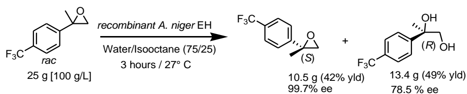
Figure 14. Preparative-scale synthesis of enantiopure para -trifluoromethyl- \alpha -methyl styrene oxide using a partially purified recombinant EH from Aspergillus niger LCP521 as biocatalyst.
