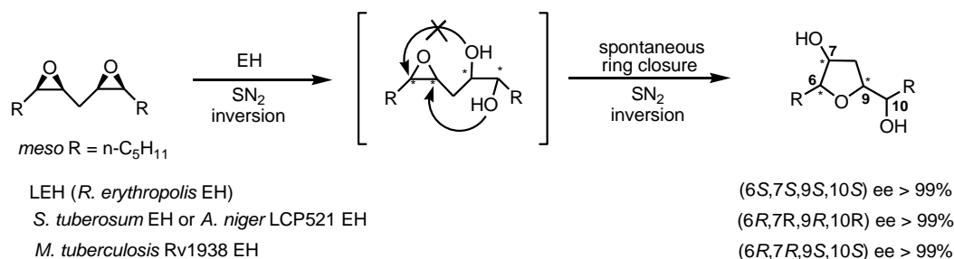
Figure 27. Stereochemical courses of epoxide-hydrolase-catalyzed hydrolysis/cyclisation cascades of 6,7:9,10-bis(epoxy)pentadecane to yield tetrahydrofurane derivatives.
