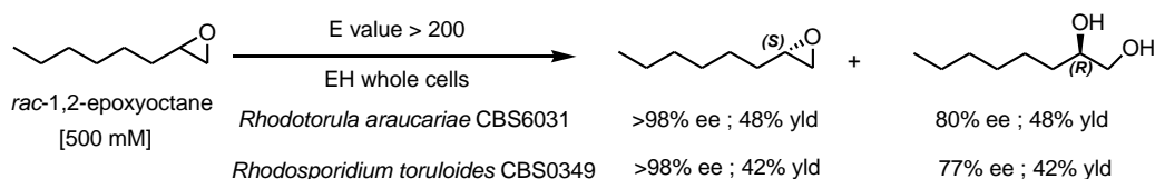
Figure 18. Kinetic resolution of 1,2-epoxyoctane at high substrate concentration with two yeast EHs
