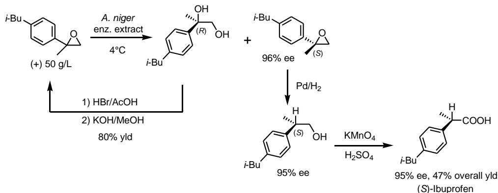
Figure 13. Preparative-scale resolution of rac -4-isobutyl- \alpha -methylstyrene oxide using an enzymatic extract of A. niger LCP521. A four step enantioconvergent procedure enabled the synthesis of ( S )-Ibuprofen.
