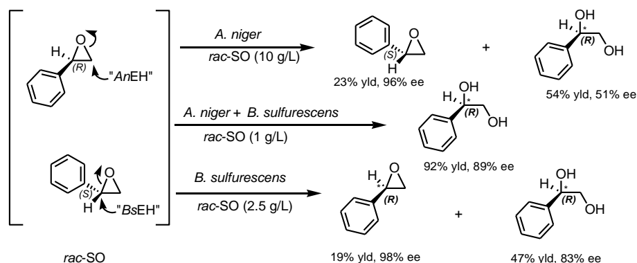
Figure 7. Biohydrolytic kinetic resolution of racemic styrene oxide ( rac -SO) catalyzed by Aspergillus niger LCP 521 ( AnEH ) and/or Beauveria sulfurescens ATCC 7159 ( BsEH ). Using both fungi together led to an enantioconvergent production of ( R )-phenyl-1,2-ethanediol.
