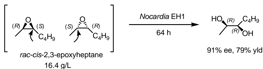
Figure 23. Deracemization of rac-cis -2,3-epoxyheptane via enantioconvergent biohydrolysis using Nocardia EH1 leading to the formation of an ( R,R )-diol.
