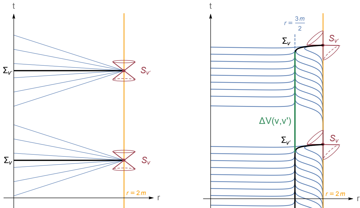
Figure 1. Left: Maximal surfaces (blue lines) inside a two-sphere in flat Minkowski spacetime. The largest is the t = \text{const.} (bold black lines) defining its inertial frame. Right: Maximal surfaces (blue lines) inside a two-sphere on the horizon of a static black hole. Apart from the transient part connecting it to the horizon, the largest surface (bold black lines) lies on the limiting surface r = 3/2m . The volume difference between the spheres S_v and S_{v'} is finite and given by (7).
