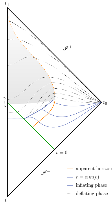
Figure 5. Speculative evolution of maximal surfaces in the case of a long-lived remnant scenario. The volume acquired during the evaporation process (continuous surfaces) deflates back to flat space (dotted surfaces). This is expected to happen in a time of order m_0^4 , during which all the information stored can be released.
