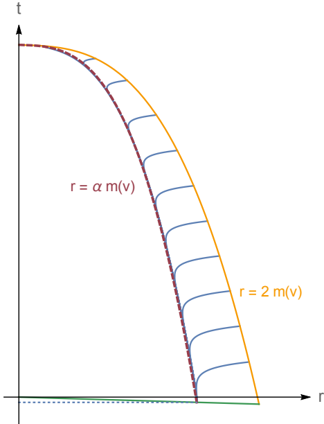
Figure 4. The surfaces defining the volume enclosed in spheres at the apparent horizon of an evaporating black hole at different times (blue lines). The limiting surface lies close to r = \alpha m(v) , with \alpha given by (9) (dashed line). Here m = 10 in Planck units.
