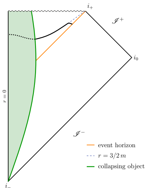
Figure 2. Penrose diagram illustrating the surface defining the volume (black curve) in the case of a black hole formed by collapse. The details of the surface in the interior of the collapsing object (dotted curve) will depend on the specific metric used to describe the latter. For Oppenheimer-Snyder and null massive shell collapses, this contribution to the volume is of the order m^3 .
