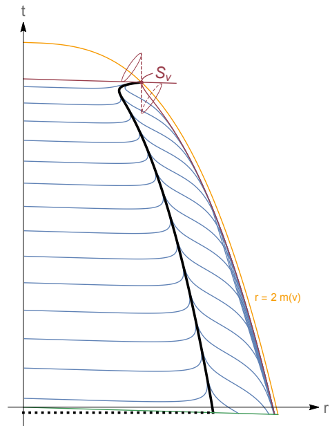
Figure 3. Eddington-Finkelstein diagram of the two families of extremal volume surfaces (blue lines) inside an evaporating black hole formed by a collapsing object. The surface defining the volume is in bold black. Note the close analogy with the static case, compare with Fig. 1.
