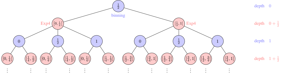
Figure 3: The structure of the efficient chaining tree in dimension d = 1 .
